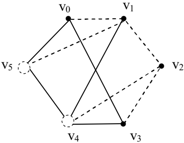
Figure 5.20 be the strong neutrosophic graph.
