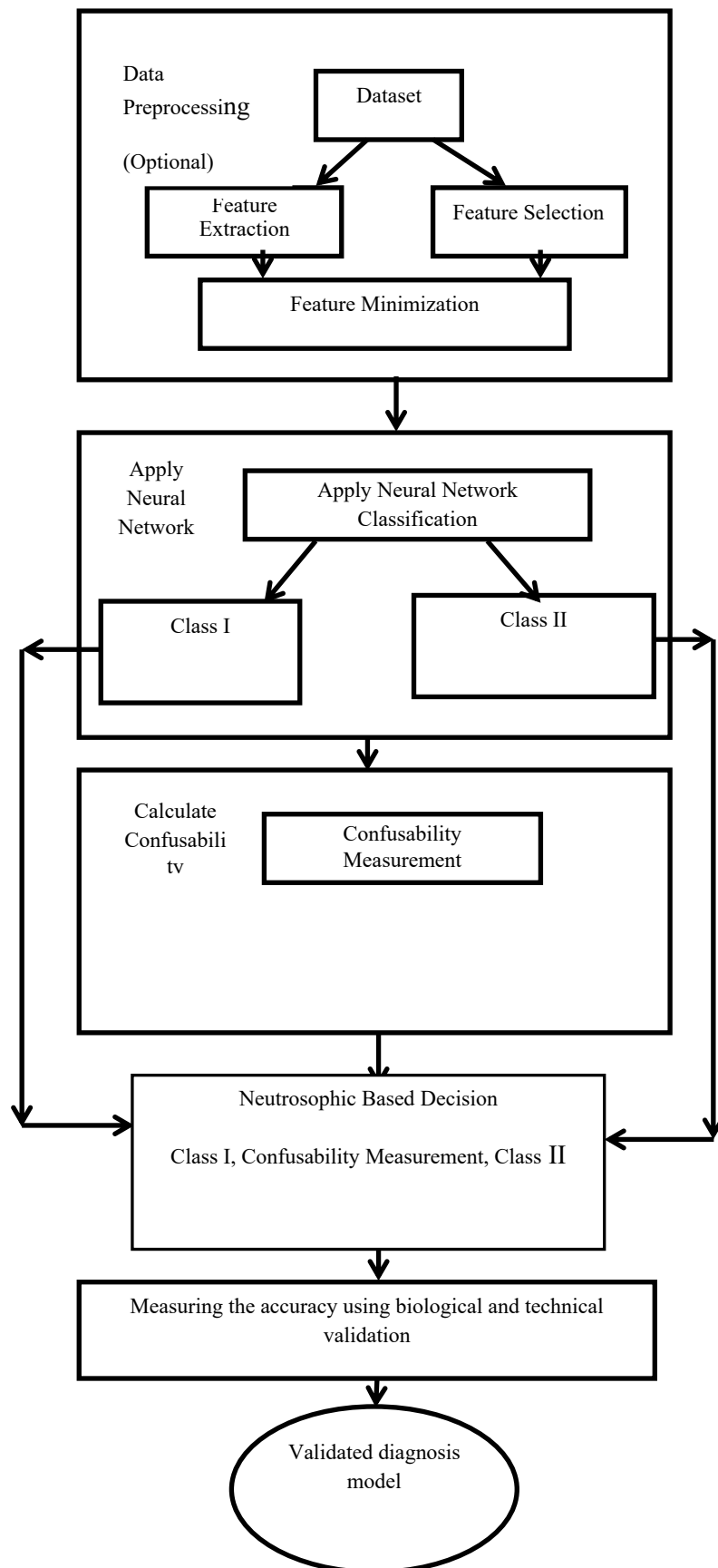
Fig. 3.2: Proposed System Architecture
