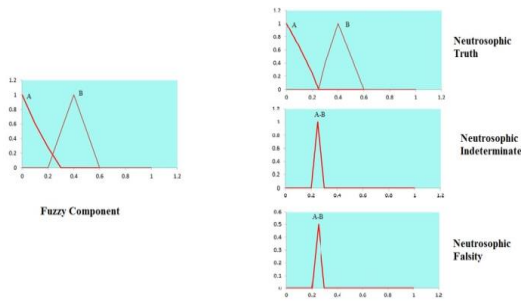
Fig. 4. Triangular Membership function for output class.
