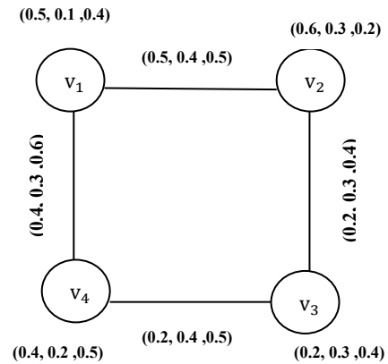
Figure 1: Single valued neutrosophic graph.
