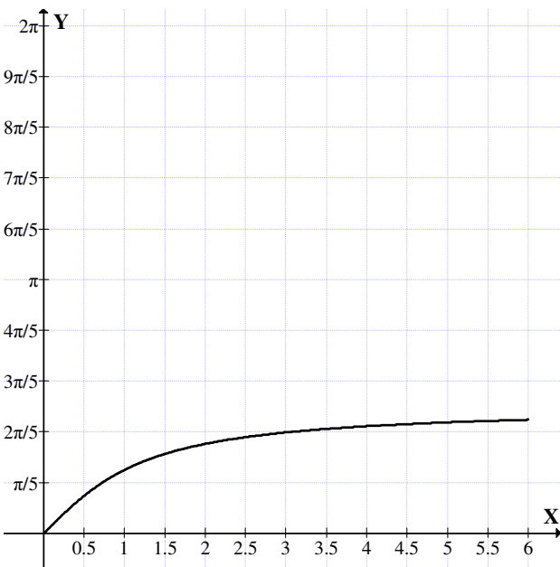
Figure 4.15: y_n = n \tan^{-1} x
