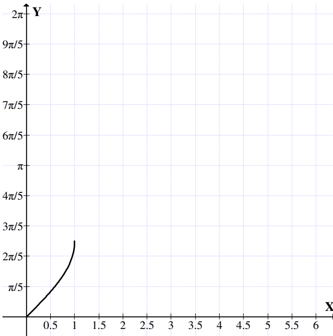
Figure 4.13: y_n = nsin^{-1}x
