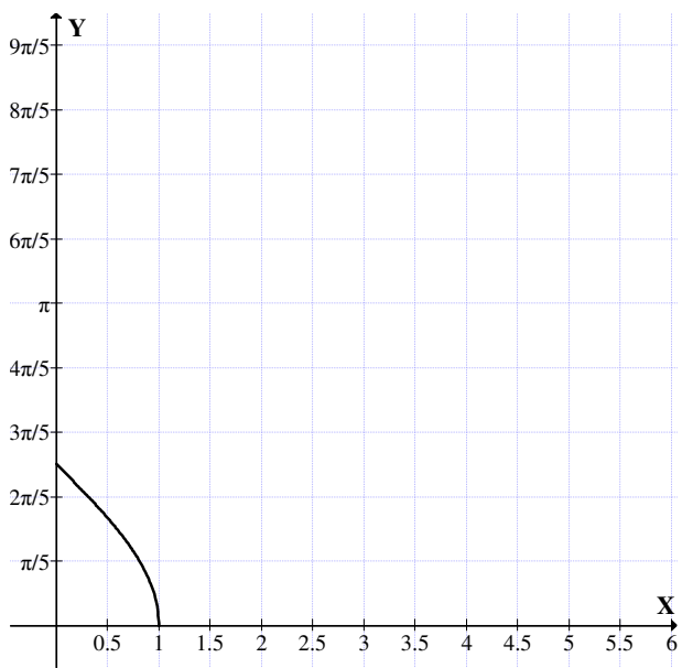
Figure 4.14: y_n = n \cos^{-1} x
