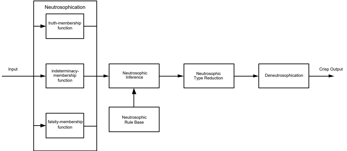
Figure 2.1: General Scheme of an INLS
