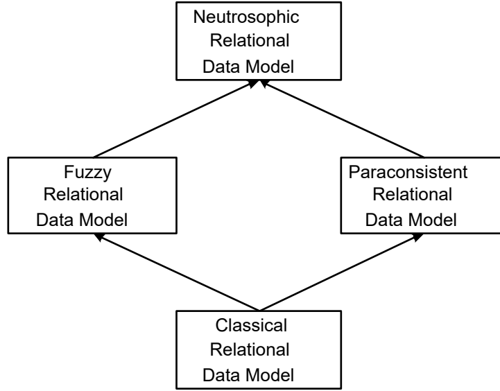
Figure 3.1: Relationship Among FRDM, PRDM, NRDM and RDM
