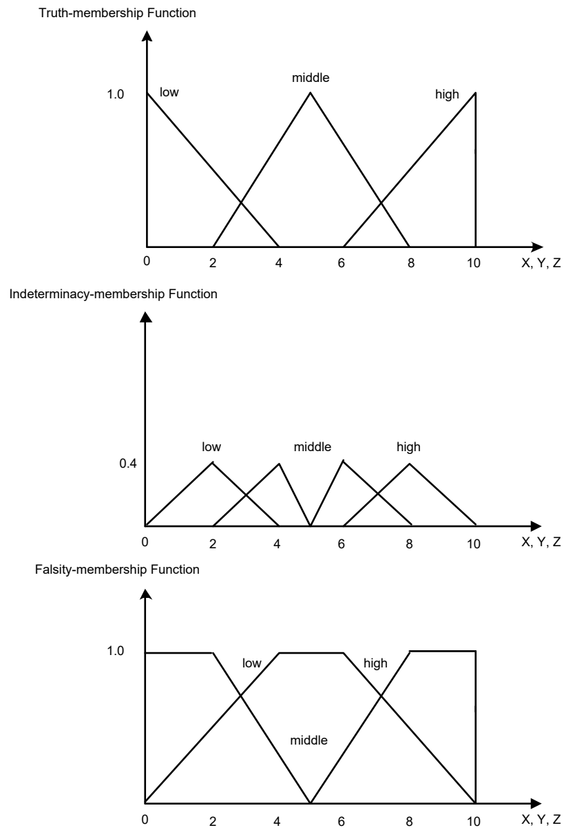
Figure 4.7: Membership functions of inputs
