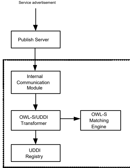
Figure 4.5: Publish service advertisement
