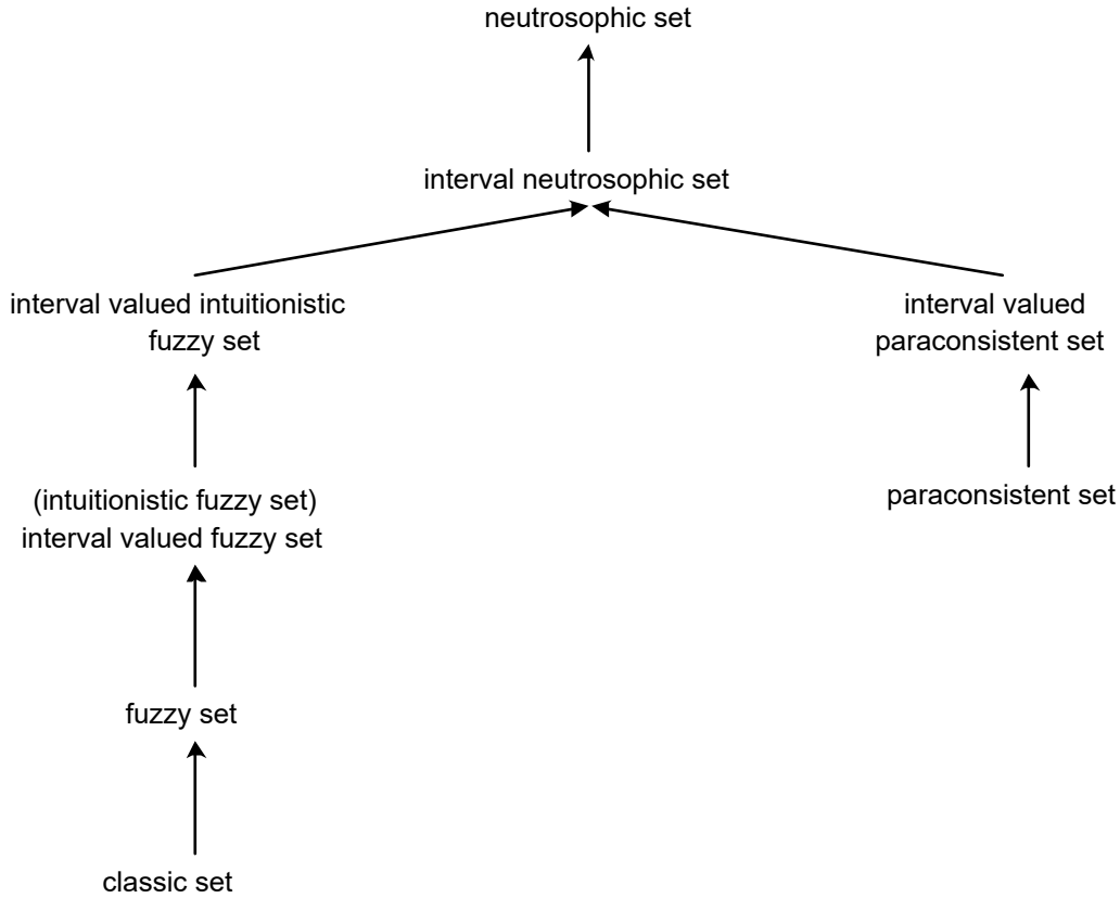
Figure 1.1: Relationship among interval neutrosophic set and other sets
