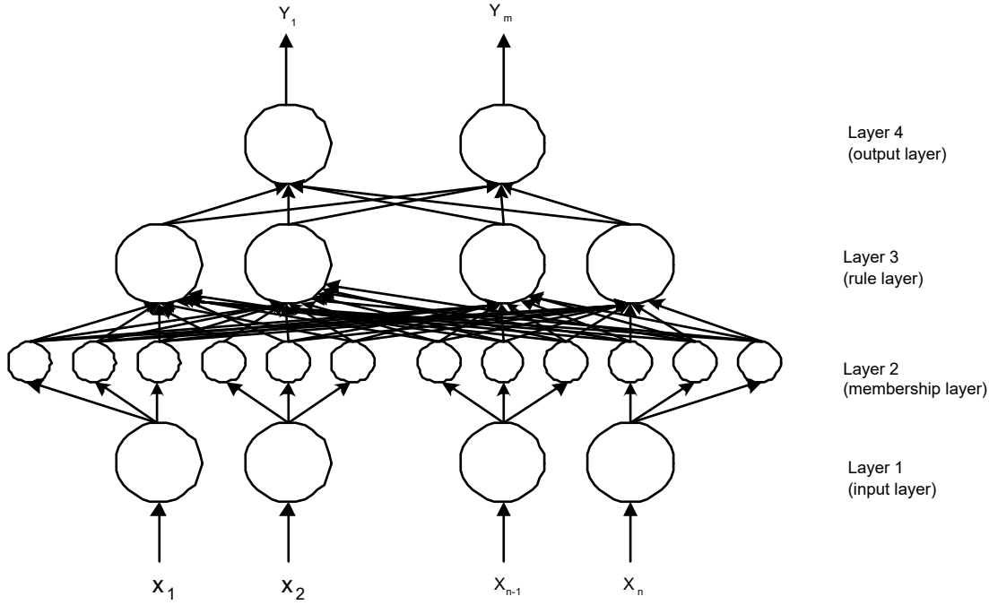
Figure 4.6: Schematic diagram of Neutrosophic Neural Network
