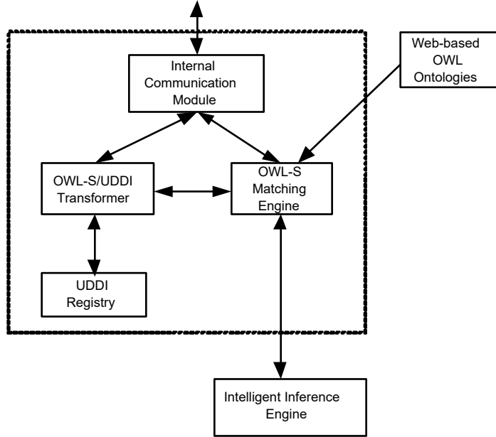
Figure 4.2: Architecture of Repository
