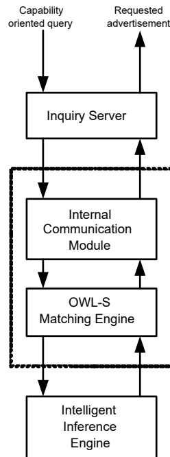
Figure 4.3: Capability oriented query
