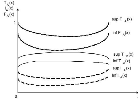
Figure 1.2: Illustration of interval neutrosophic set in R^1
