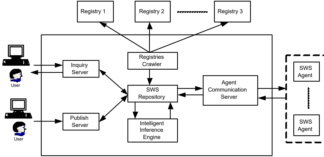
Figure 4.1: Architecture of the Extensible Soft SWS Agent
