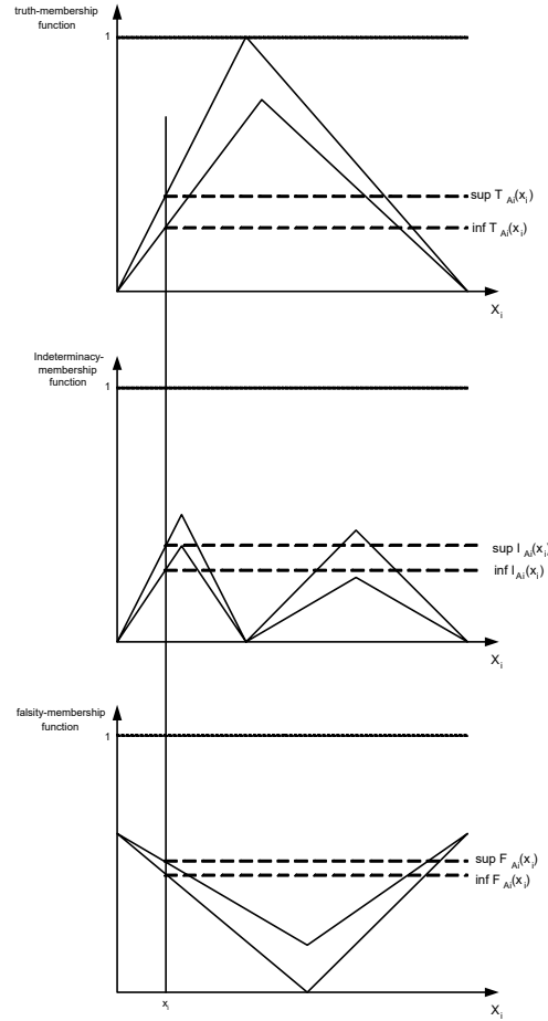
Figure 2.2: Conceptual Diagram for Neutrosophication of Crisp Input
