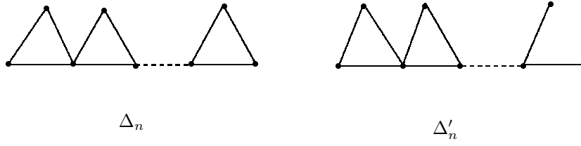
Figure 2 Triangular snake graph (\Delta_n)
