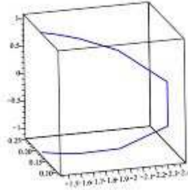
Figure 5 \Omega_1\Omega_2B -Smarandache curve
