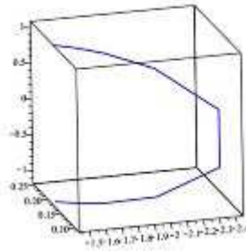
Figure 3 \Omega_1B -Smarandache curve
