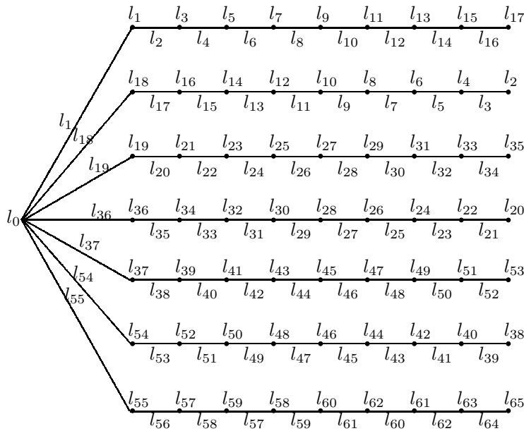
Fig.2.1 S_{7,9}
