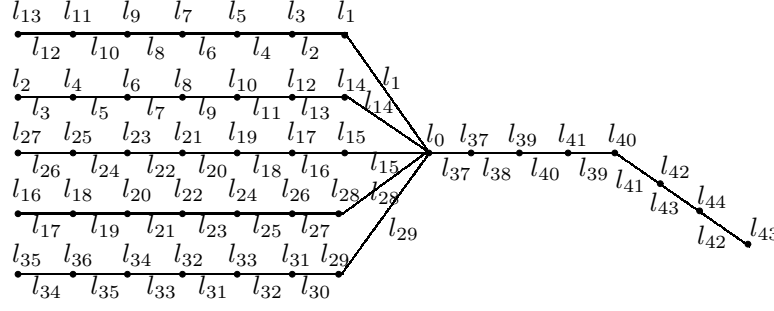
Fig.3.1 S_{5,7} @ P_7
