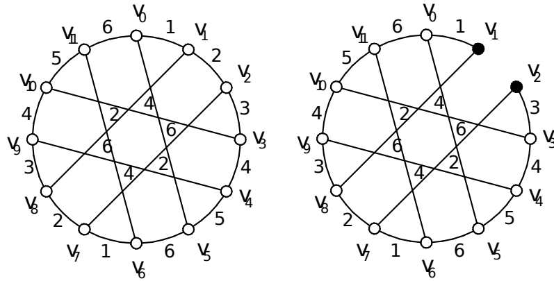
Figure 7 Assignment of colors in C(12, 1, 5) .
