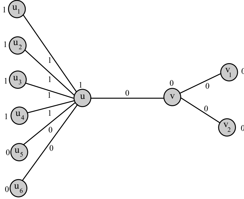
Figure 6 Graph B_{6,2}
