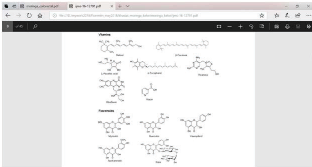
Figure 1. Chemical structures of bioactive compounds in MO. After Leone et al. [5]
