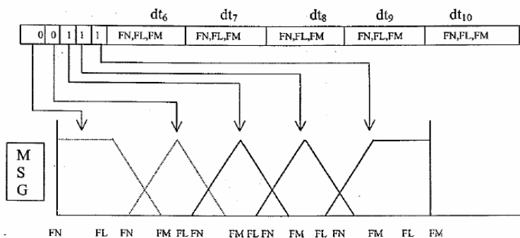
Figure 3.18: HGFCFA Design for Population string-8
