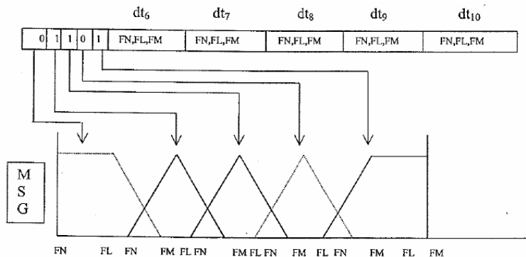
Figure 3.18: HGFCFA Design for Population string-8
