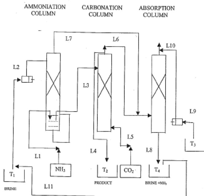
Figure 3.1: Chemical Plant
