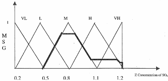
Figure 5.14: Aggregated output and defuzzification for the concentration of SO_x
