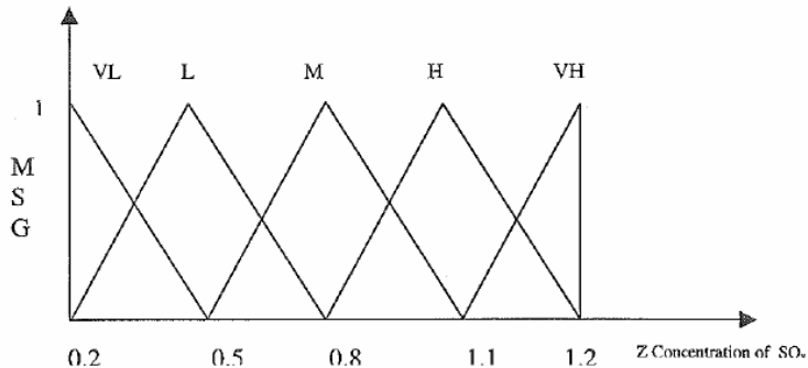
Figure 5.6: Concentration of \text{SO}_x output parameter
