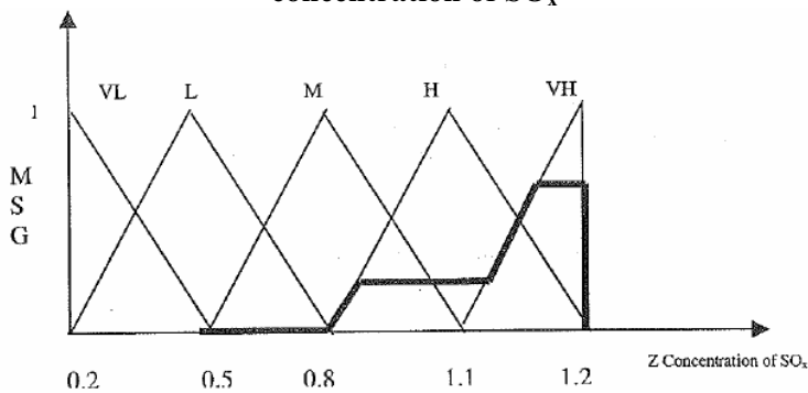
Figure 5.22: Aggregated output and defuzzification for the concentration of SO_x
