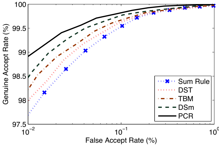
Figure 17.2: ROC of the proposed fusion framework with Sum rule, DS theory fusion, TBM, DSsm and PCR rule for multiclassifier face verification .
