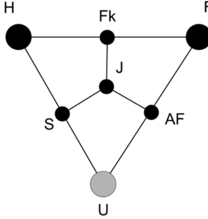
Figure 11.7: Relations among threat values (UNKNOWN is specific) where Fk \triangleq \text{FAKER} , J \triangleq \text{JOKER} , S \triangleq \text{SUSPECT} and AF \triangleq \text{ASSUMED\_FRIEND} .
