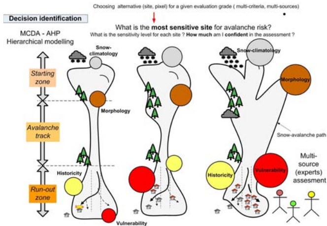
Figure 23.42: Decision context: ranking avalanche prone areas according hazard and vulnerability related criteria.
