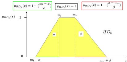
Figure 23.15: Fuzzy interval L - R .
