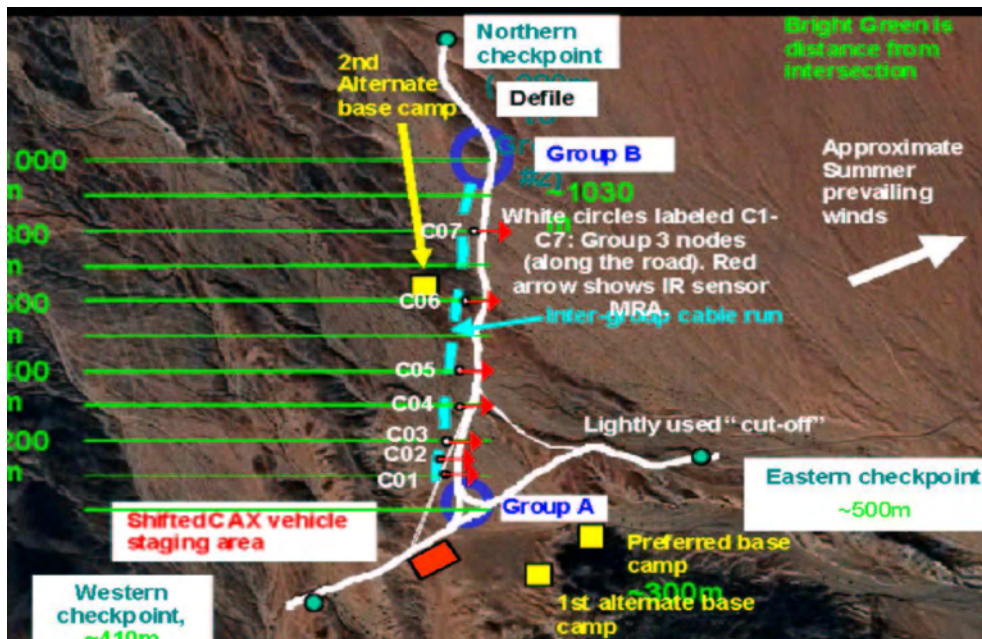
Figure 18.7: Sensor node distribution at Twenty nine Palms, CA
