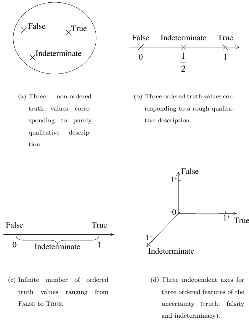
Figure 16.4: Supplementary truth values for representing indeterminacy.
