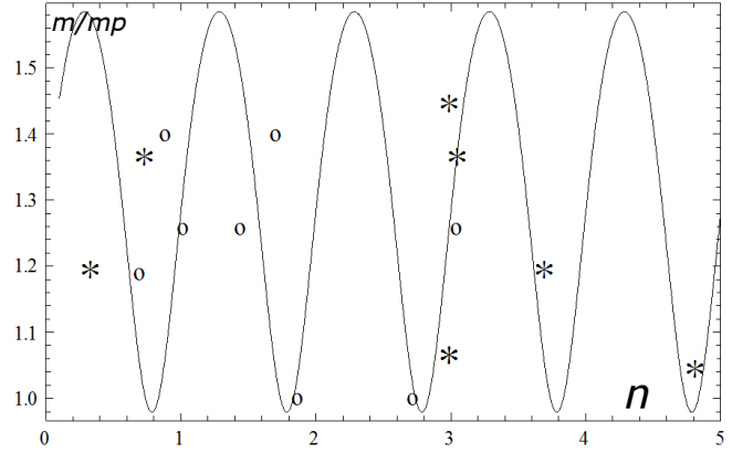
Fig. 2: Comparison of baryon masses calculated from Eq.(8) as a function of confined flux n , with data from Tables 1 and 2 for octet (open circles) and decuplet particles ( m_i used, stars). The phenomenological Eq.(4) provides values for n as a function of mass and moment, and the relation between these quantities (data points) agrees quite well with the field-theoretical calculations (curve) of mass as function of n from Eq. (8). Nucleons are on the basis of the figure.
