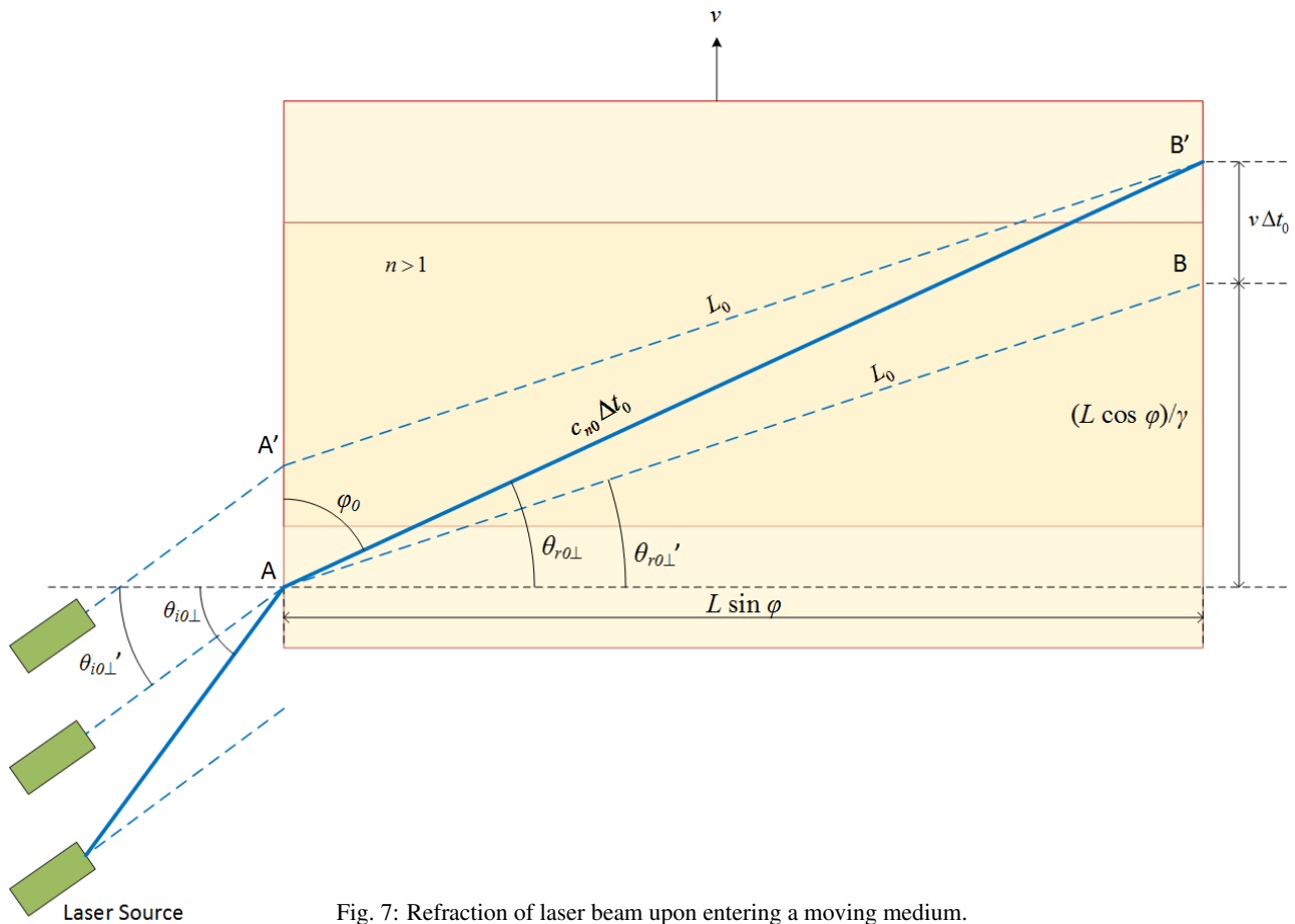
Fig. 7: Refraction of laser beam upon entering a moving medium.
