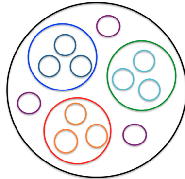
Fig. 4: A simple sketch of the innermost three layers of the entire space that is structured hierarchically. The black circle represents the mother universe. Our black hole universe is coded as red, in which three child universes ( i.e. star-like or supermassive black holes) were drawn. Parallel to our universe, there are sister universes. Here two adult sister universes (blue and green circles) and three little sister universes (brown circles). The adult sister universes have also their child or baby universes, but the little sister universes are too young to have their babies.
