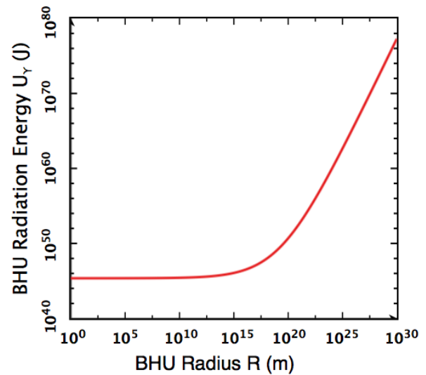
Fig. 9: Radiation energy of the black hole universe. As a hot star-like black hole with T_s = 10^{12} K expands to the size of the present universe and cools down to \sim 2.725 K, its radiation energy first remains as a constant and then rapidly increases with radius when it grows into a supermassive black hole with radius greater than about thousand billions of kilometers or mass greater than about hundred billions of solar masses.
