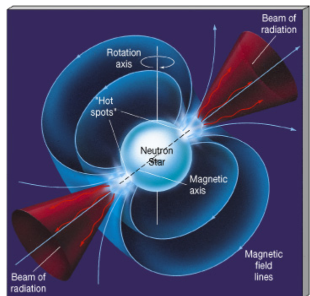
Fig. 1: A sketched diagram for the lighthouse model of pulsars as fast rotating neutron stars (Credit: www.pas.rochester.edu/afrank/A105 ). Charged particles, accelerated by the magnetism of the neutron star, flow along the magnetic field lines, producing radio radiation that beams outward.
