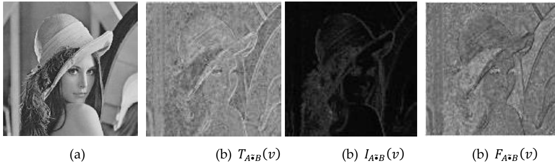
Fig.3.3.2 (II): Applying the neutrosophic closing operator: a) Original image b) Neutrosophic closing components in type II \langle T_{A\tilde{\bullet}B}(v), I_{A\tilde{\bullet}B}(v), F_{A\tilde{\bullet}B}(v) \rangle respectively.
