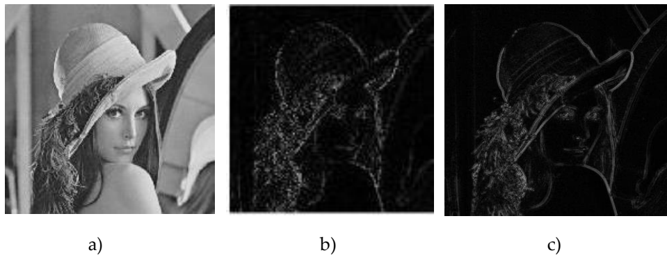
Fig. 3.7.2: Neutrosophic Outline Boundary: a) Original Image, b) Neutrosophic Outline Boundary Filtered Image, c) Neutrosophic Outline Boundary Filtered Image
