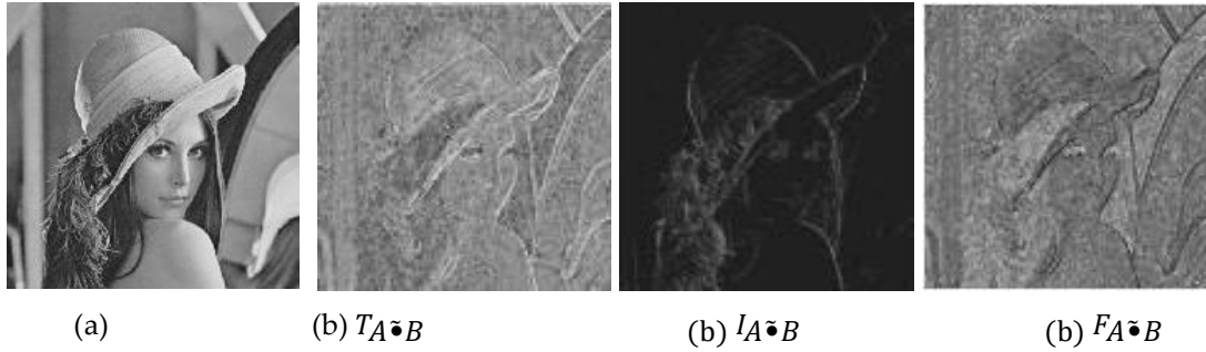
Fig. 3.3.2 (I): Applying the neutrosophic closing operator: (a) Original image (b) Neutrosophic closing components in type I \langle T_{A\tilde{\bullet}B}, I_{A\tilde{\bullet}B}, F_{A\tilde{\bullet}B} \rangle respectively.
