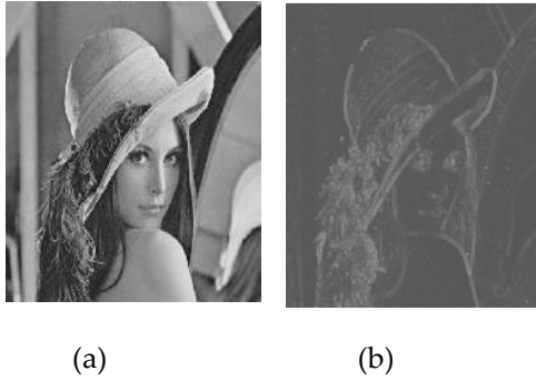
Fig. 3.7.1.2 (I): Applying the Neutrosophic Fuzzy External Boundary: a) Original Image
