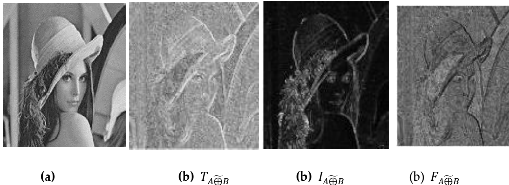
Fig 3.1.1 (I): Applying the NFD operator: (a) Original image, (b) Neutrosophic Fuzzy components of the dilated image in type I \langle T_{A \widetilde{\oplus} B}, I_{A \widetilde{\oplus} B}, F_{A \widetilde{\oplus} B} \rangle respectively.
