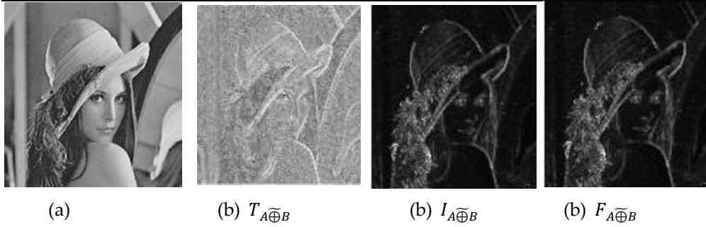
Fig.3.1.1 (II): Applying the neutrosophic dilation operator: a) Original image b) Neutrosophic Fuzzy components of the dilated image in type II \langle T_{A\oplus B}, I_{A\oplus B}, F_{A\oplus B} \rangle respectively.
