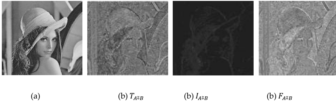
Fig.3.3.1 (I): Applying the neutrosophic fuzzy opening operator: (a) Original image. (b) Neutrosophic fuzzy opening components in type I \langle T_{A\tilde{B}}, I_{A\tilde{B}}, F_{A\tilde{B}} \rangle respectively.
