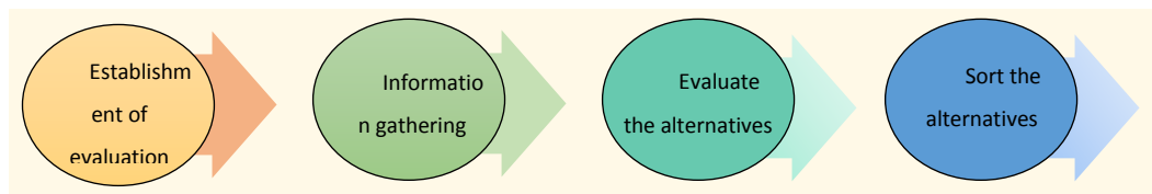
Figure 1. Proposed model.
