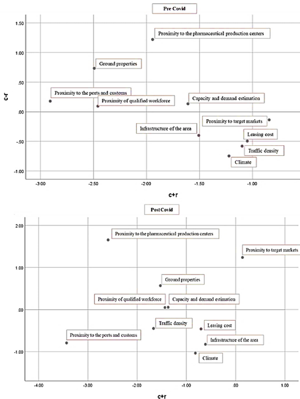
Fig. 1. Causal diagrams.
