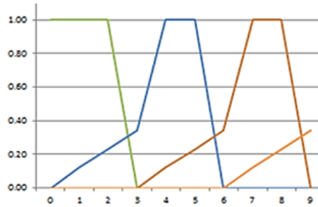
Fig. 5. Different tolerance varieties of mutated fuzzimetric sets: a. triangular; b. minimize tolerance for all sets (MINMIN); c. minimize PO & PS, maximize PM & PB tolerances; d. maximize PO & PS, minimize PM & PB tolerance; e. maximize tolerance for all sets (MAXMAX).
