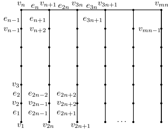
Figure 2 Uniform k -distant tree
