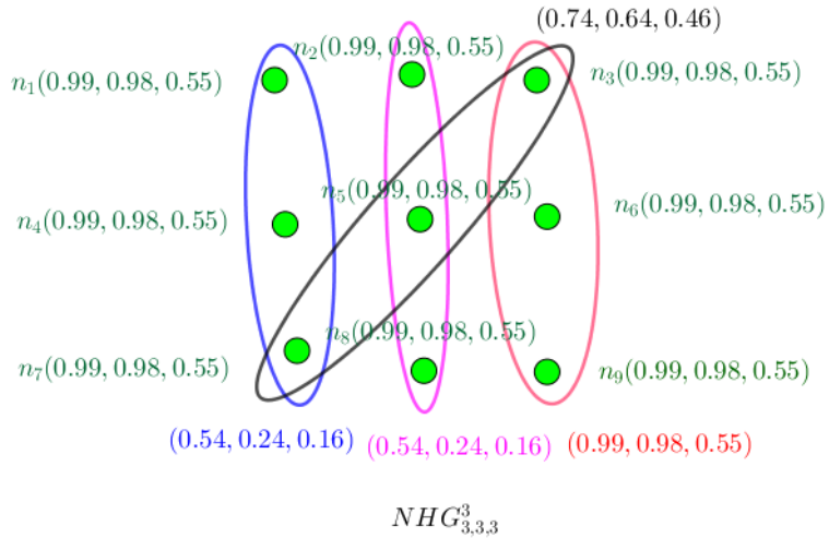
Figure 8. Vertices are suspicions about choosing them.
