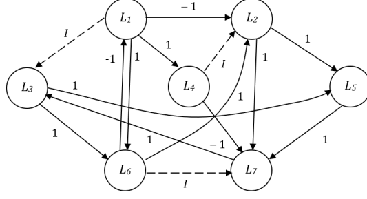
Figure 2: Neutrosophic directed graph for simple NCM
