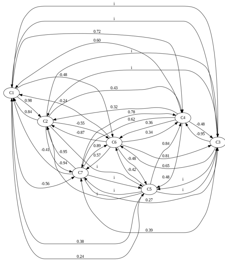
Figure 7: Neutrosophic directed graph
