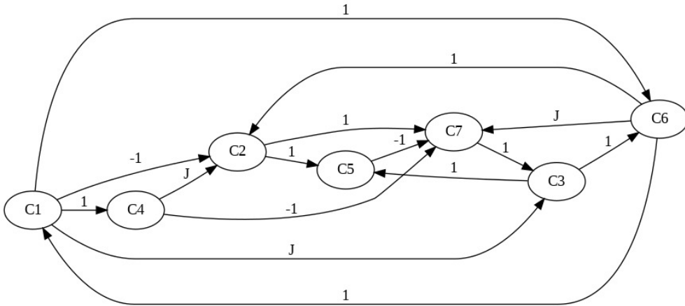
Figure 10: Visualization of the neutrosophic graph
