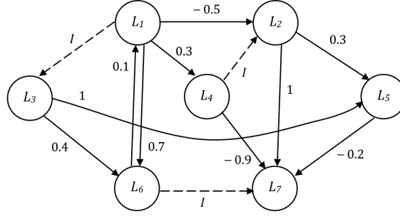
Figure 1: An illustration of the neutrosophic directed graph
