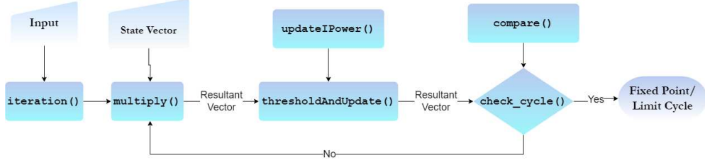
Figure 4: Flowchart of the NCM package
