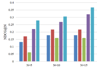
(a)NDCG@N
