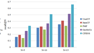
(c)recall@N
