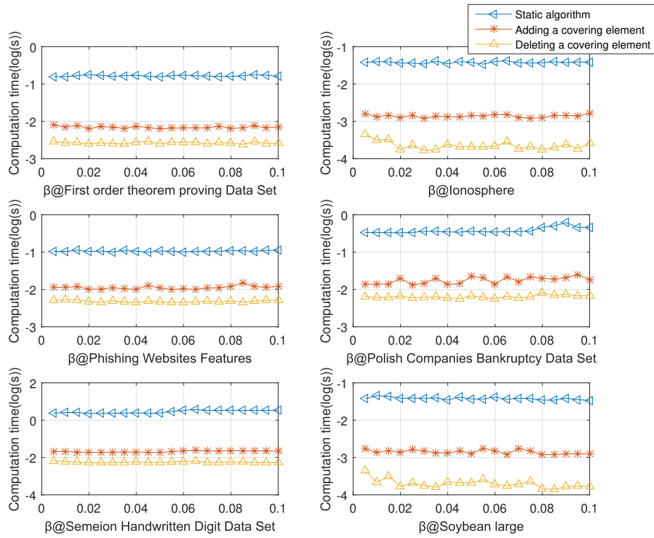
Figure 9: Comparison of Algorithm 1,2 and 3
