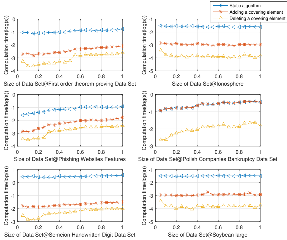
Figure 8: Comparison of Algorithm 1,2 and 3
