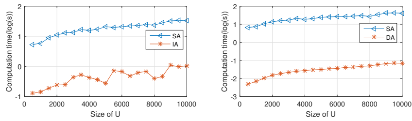
Figure 4: Comparison of Algorithm 1,2 and 3 with the percentage of reducible element is 95%
