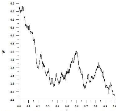
Figure 11: Discretized Brownian path for 1000 generation.
