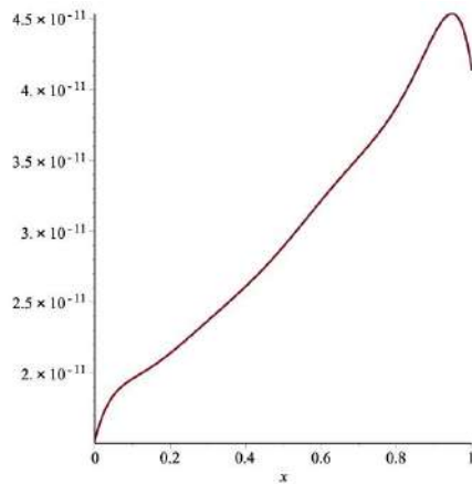
Figure 7: Graph of u(x, t) - u_{NM}(x, t) for t = 2.9 and N = M = 10
