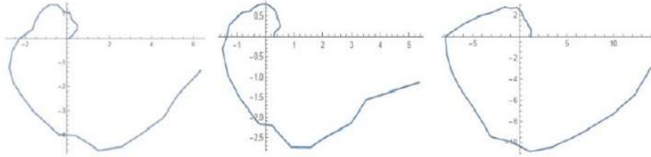
Figure 3: Wrapped Shanker distribution for n = 30 , \lambda = 0.5 , \lambda = 1 , and \lambda = 2 respectively
