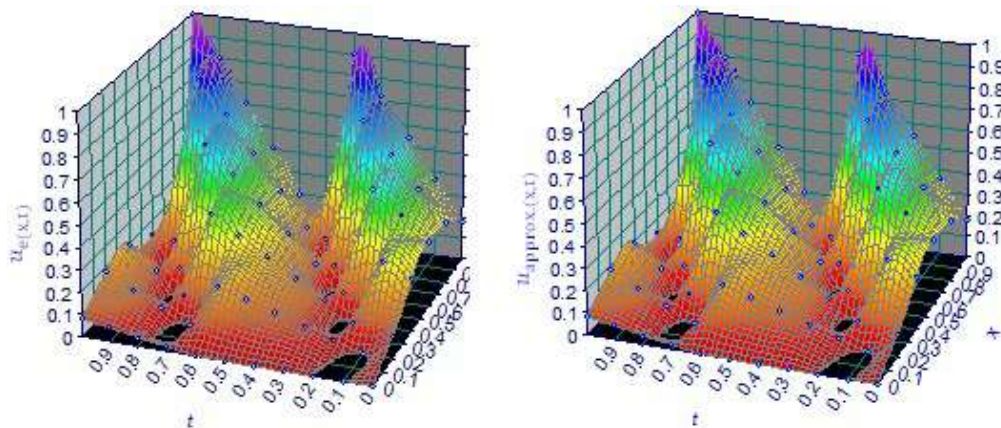
Figure 7: Comparison between the approximate solution of problem (39)-(40) using HAM up to 4-terms and the exact solution.
