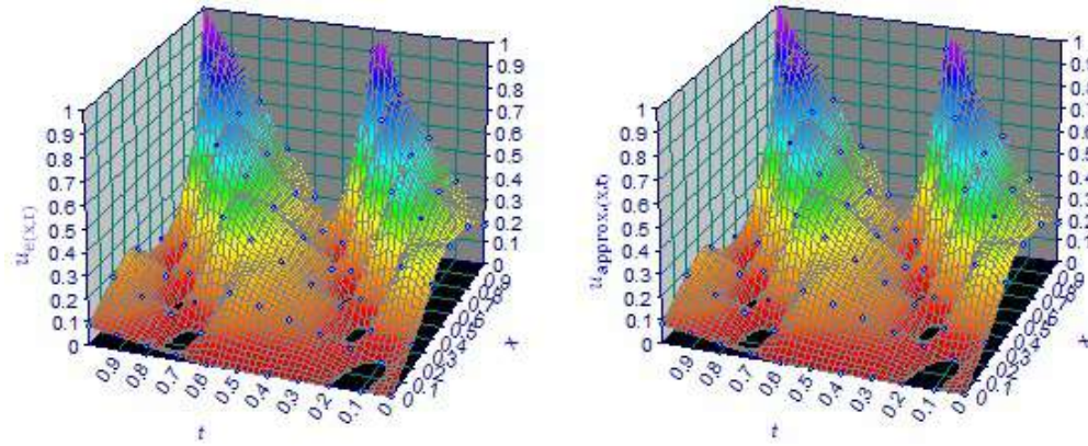
Figure 2: Comparison between the approximate solution of problem (33)-(34) using ADM up to 4-terms and the exact solution.
