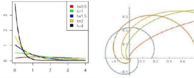
Figure 1: The Linear and Circular representation for the PDF of wrapped Shanker distribution for different values of \lambda
