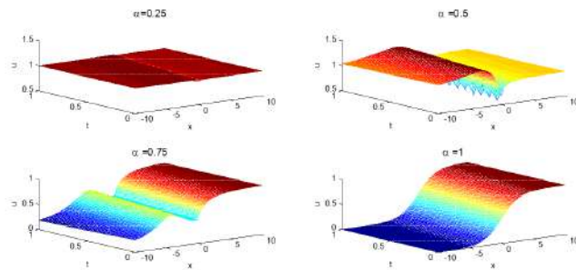
Figure 1: The solution u_3(x, t) if \lambda = -1, a_0 = 1/2, a_1 = \sqrt{2}
