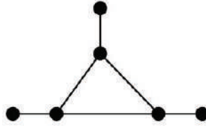
Figure 1: 3-cycle graph
