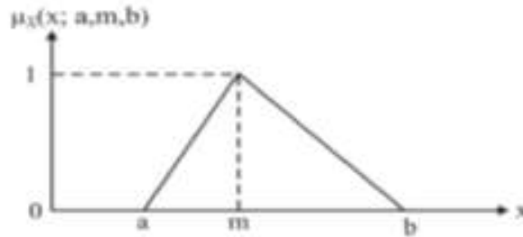
Figure 1: Triangular Fuzzy Number A
