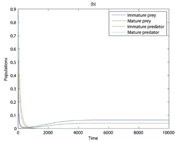
(b) Time series of the solution of System (2) for the values in eq. (13) at a_4 = 0.8 , approaches to E_1 = (0.064, 0.039, 0, 0) in the positive quadrant of xy -plane
