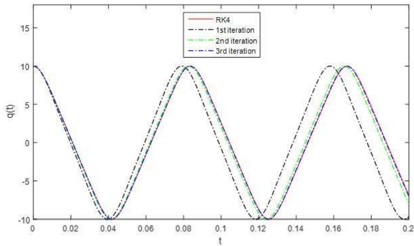
Figure 4: Comparison between approximated solutions and corresponding numerical one for a = b = c = 1 and A_0 = 10 .
