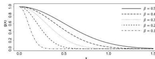
Figure 1: The detection functions of the half-normal models.
