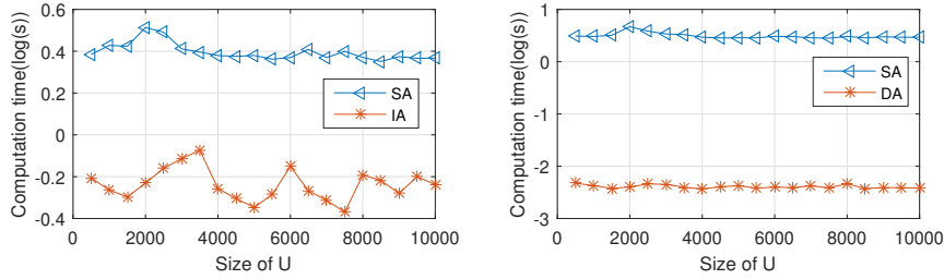
Figure 2: Comparison of Algorithm 1,2 and 3 with the percentage of reducible element is 5%
