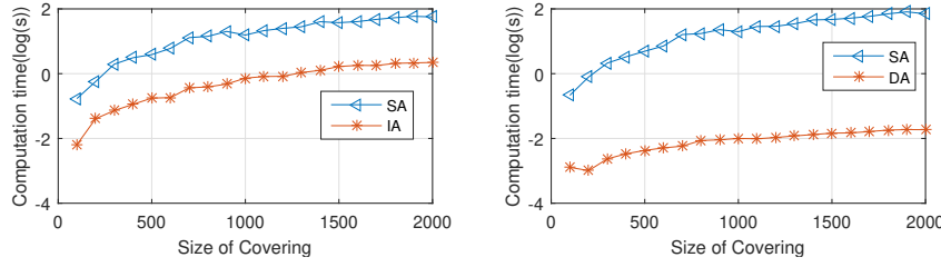
Figure 7: Comparison of Algorithm 1,2 and 3 with the percentage of reducible element is 95%
