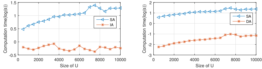
Figure 3: Comparison of Algorithm 1,2 and 3 with the percentage of reducible element is 50%
