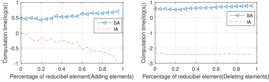
Figure 1: Comparison of Algorithm 1,2 and 3
