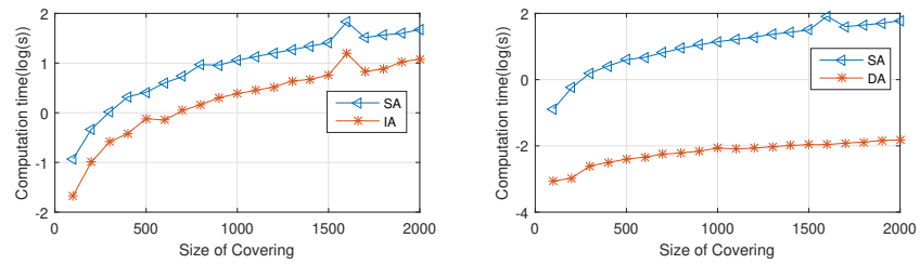
Figure 5: Comparison of Algorithm 1,2 and 3 with the percentage of reducible element is 5%
