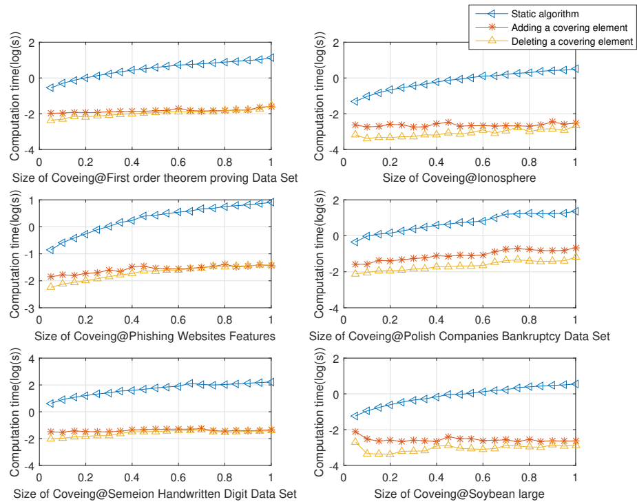
Figure 10: Comparison of Algorithm 1,2 and 3
