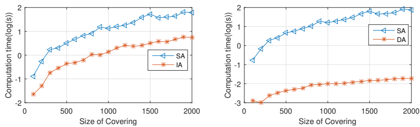
Figure 6: Comparison of Algorithm 1,2 and 3 with the percentage of reducible element is 50%
