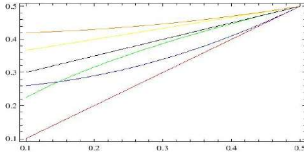
Figure 2: Graph representing inequality chain (16)
