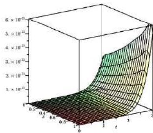
Figure 5: Graph of u(x, t) - u_{exp}(x, t) for N = M = 10
