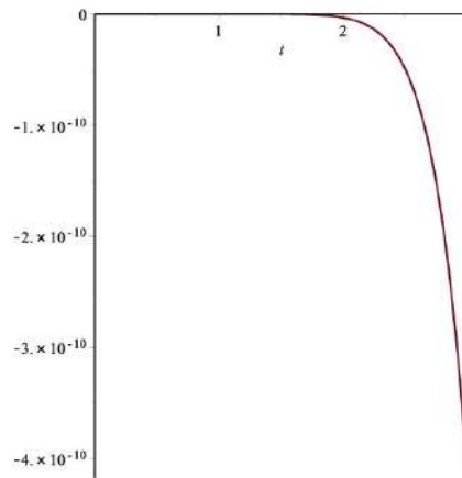
Figure 8: Graph of a(t) - a_{app}(t) for N = M = 10
