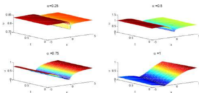
Figure 3: The solution u_{11}(x, t) if \lambda = 0 , a_0 = 1/3 , a_1 = \sqrt{2}
