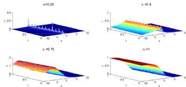
Figure 2: The solution u_9(x, t) if \lambda = -1, a_0 = 1/2, a_1 = -\sqrt{2}
