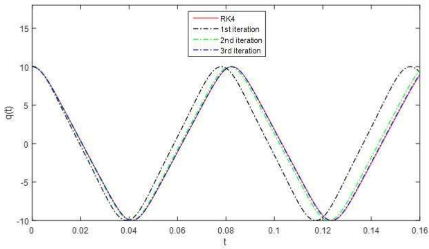
Figure 5: Comparison between approximated solutions and corresponding numerical one for a = 5 , b = 3 , c = 1 and A_0 = 10 .
