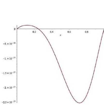
Figure 3: Graph of u(x, t) - u_{NM}(x, t) for t = 0.1 and N = M = 10
