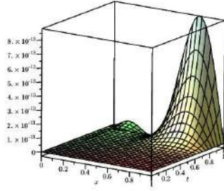
Figure 1: Graph of u(x, t) - u_{NM}(x, t) for N = M = 10
