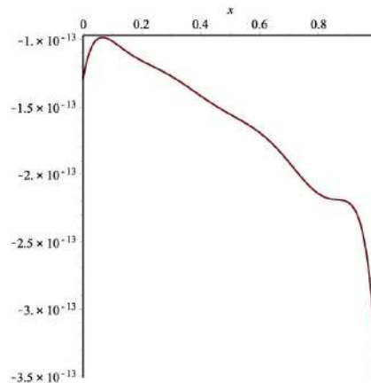
Figure 6: Graph of u(x, t) - u_{NM}(x, t) for l = 1 and N = M = 10
