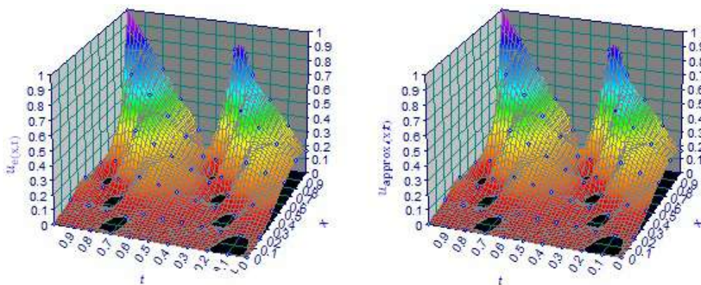
Figure 3: Comparison between the approximate solution of problem (35) -(36) using HAM up to 4-terms and the exact solution.
