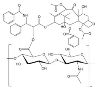
Figure 1: The HA-PTX conjugate molecular structure.
