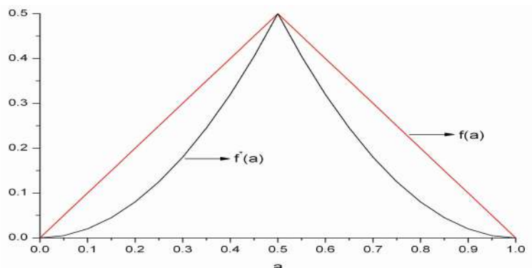
Figure 1: Graph of f(a) and f^*(a) over [0, 1]
