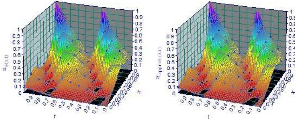
Figure 1: Comparison between the approximate solution of problem (33)-(34) using HAM up to 4-terms and the exact solution.
