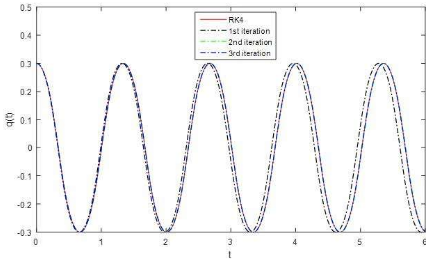
Figure 3: Comparison between approximated solutions and corresponding numerical one for a = 48.0611 , b = -543.1630 , c = 2223.874 and A_0 = 0.3 .
