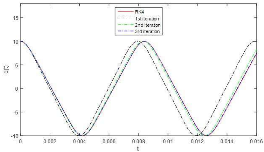
Figure 6: Comparison between approximated solutions and corresponding numerical one for a = 1 , b = 10 , c = 100 and A_0 = 10 .
