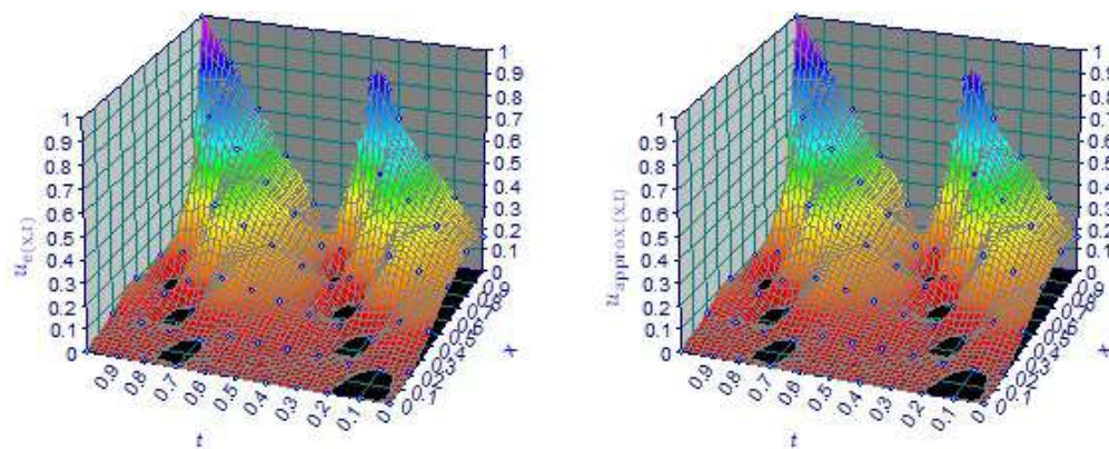
Figure 4: Comparison between the approximate solution of problem (35)-(36) using ADM up to 4-terms and the exact solution.
