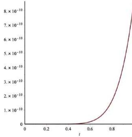
Figure 4: Graph of a(t) - a_{app}(t) for N = M = 10
