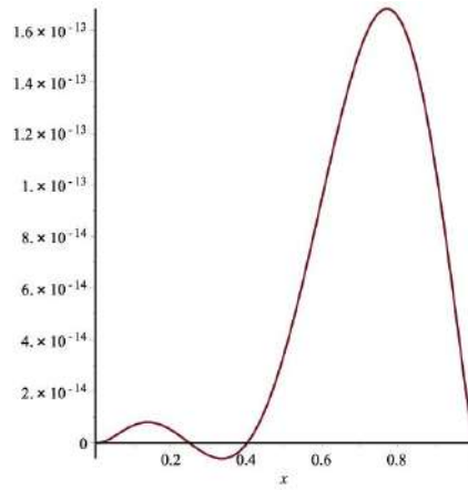
Figure 2: Graph of u(x, t) - u_{NM}(x, t) for t = 0.9 and N = M = 10
