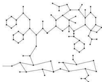
Figure 2: The corresponding molecular graph G_1 : n = 1 .
