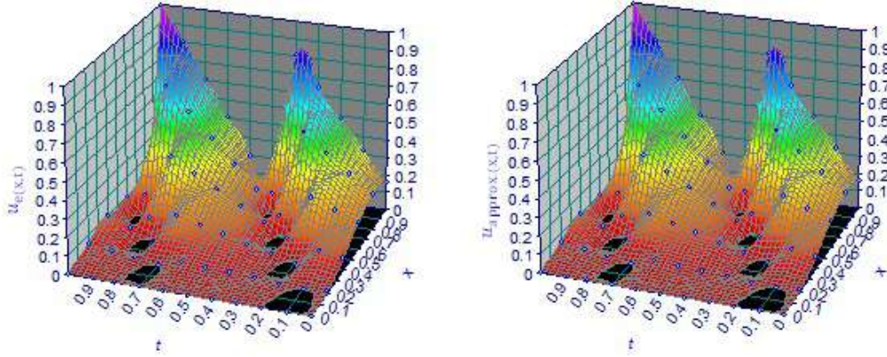
Figure 5: Comparison between the approximate solution of problem (37)-(38) using HAM up to 4-terms and the exact solution.
