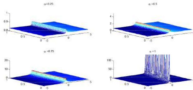
Figure 4: The solution u_{12}(x, t) if \lambda = 0, a_0 = 1/3, a_1 = \sqrt{2}
