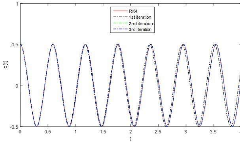
Figure 2: Comparison between approximated solutions and corresponding numerical one for a = 96.4221 , b = -364.1738 , c = 2223.874 and A_0 = 0.5 .
