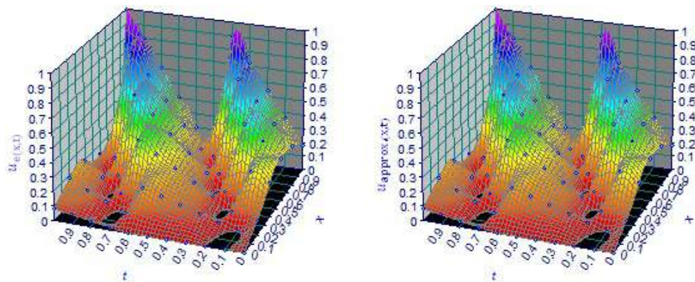
Figure 8: Comparison between the approximate solution of problem (39)-(40) using ADM up to 4-terms and the exact solution.
