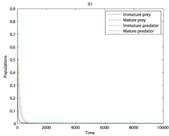
(c) The solution of system (2) for the values in eq. (13) at a_4 = 0.832 , approaches E_0 = (0, 0, 0, 0) .
