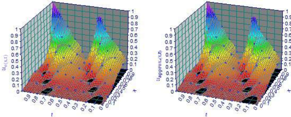
Figure 6: Comparison between the approximate solution of problem (37)-(38) using ADM up to 4-terms and the exact solution.
