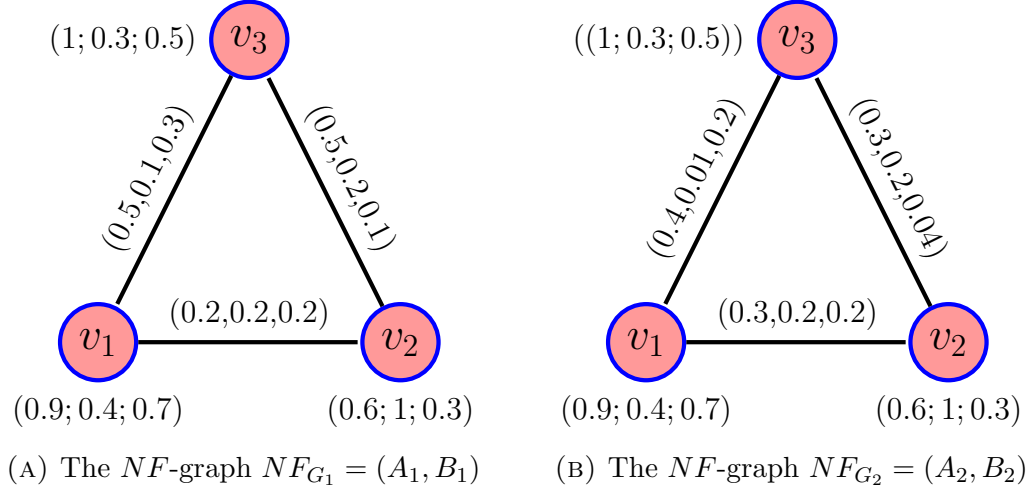
FIGURE 2. Two NF -graphs.
