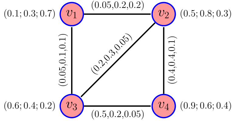
FIGURE 4. NF -graph NF_G = (A, B)
