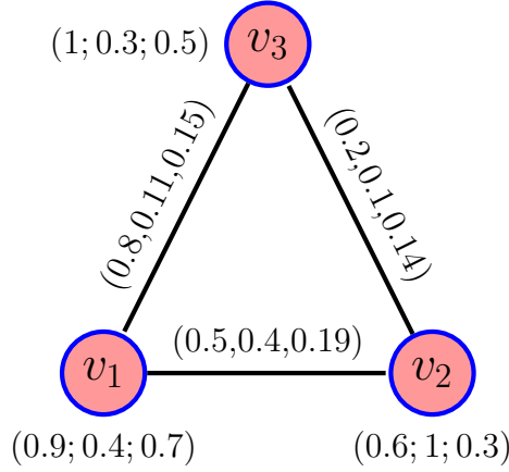
FIGURE 3. The NF -graph NF_G = NF_{G_1} \oplus NF_{G_2}
