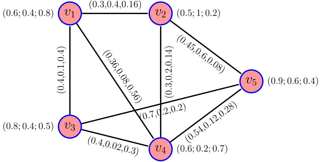
FIGURE 5. NF -graph NF_G = (A, B)
