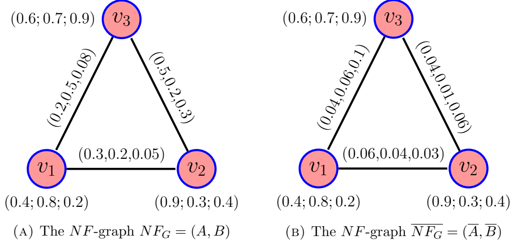
FIGURE 1. Two NF -graphs one is the complement of the other.
