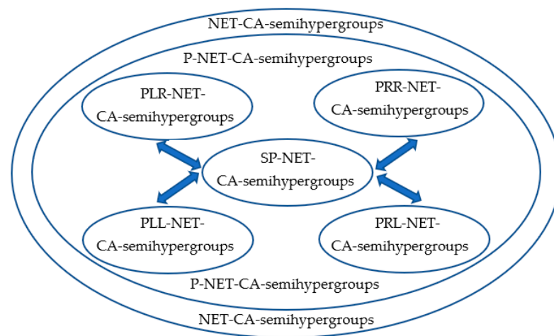
Figure 15. The relations among various P-NET-CA-semihypergroups.
