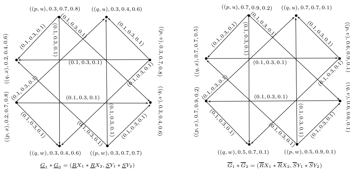
Figure 10. Neutrosophic rough digraph G = (\underline{G}_1 * \underline{G}_2, \overline{G}_1 * \overline{G}_2) .
