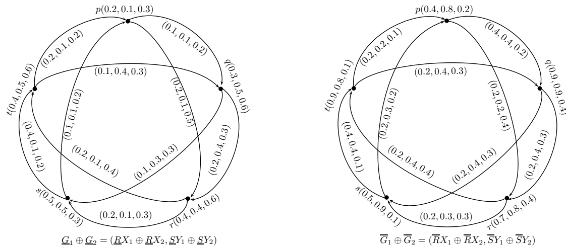
Figure 5. Neutrosophic rough digraph G = (\underline{G}_1 \oplus \underline{G}_2, \overline{G}_1 \oplus \overline{G}_2) .
