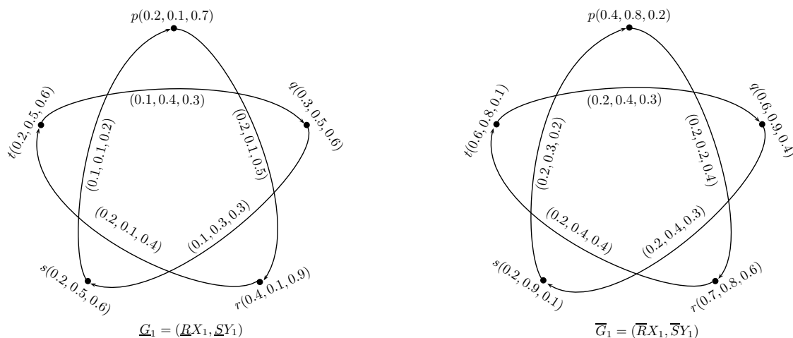
Figure 1. Neutrosophic rough digraph G_1 = (\underline{G}_1, \overline{G}_1) .
