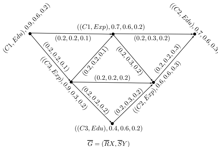
Figure 13. Neutrosophic Digraph \overline{G} = (\overline{RX}, \overline{SY})
