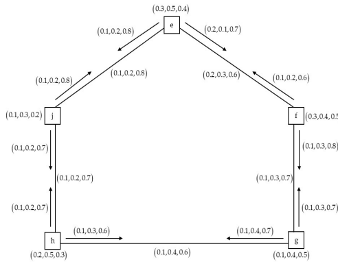
Fig. 3. SVNIG \xi in Example 3.
