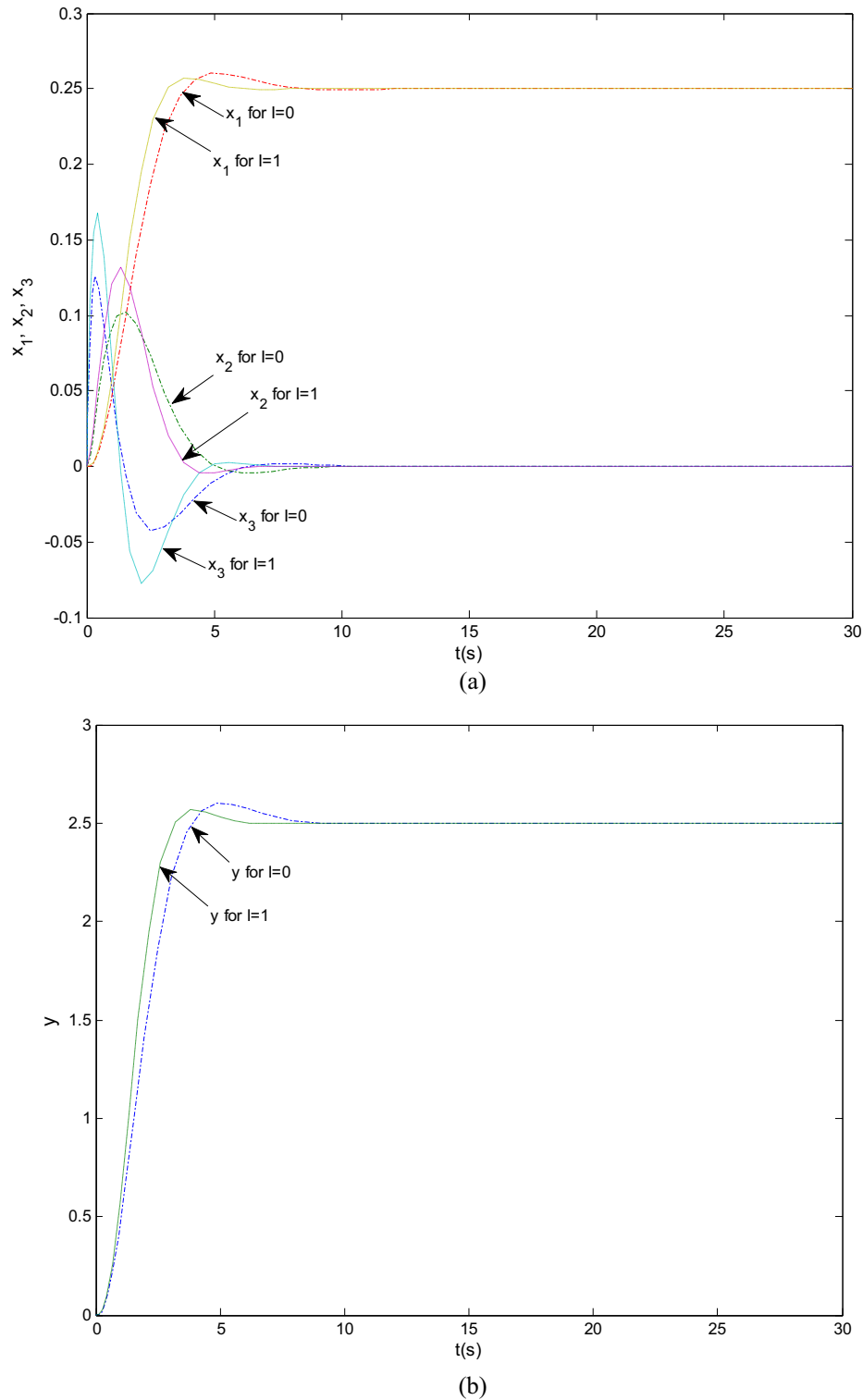
Fig. 5. Step responses of the neutrosophic state feedback system corresponding to \mathbf{K} = [4, 5, 3] and the indeterminate plant with I = 0, 1 . (a) State variable responses; (b) output responses.
