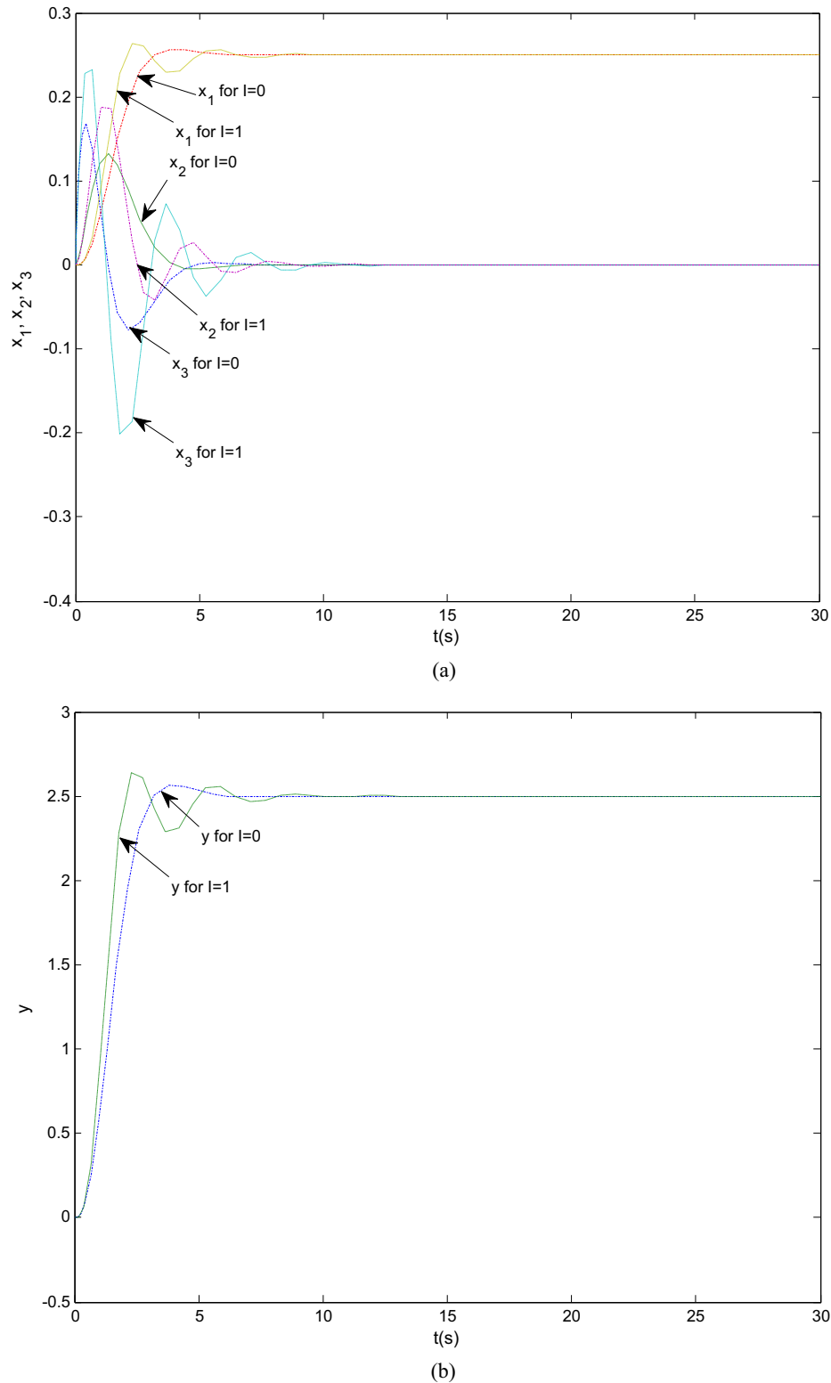
Fig. 3. Step responses of the traditional state feedback system (a special case of the neutrosophic state feedback system) corresponding to \mathbf{K} = [4, 4, 1] and the indeterminate plant with I = 0, 1 . (a) State variable responses; (b) output responses.
