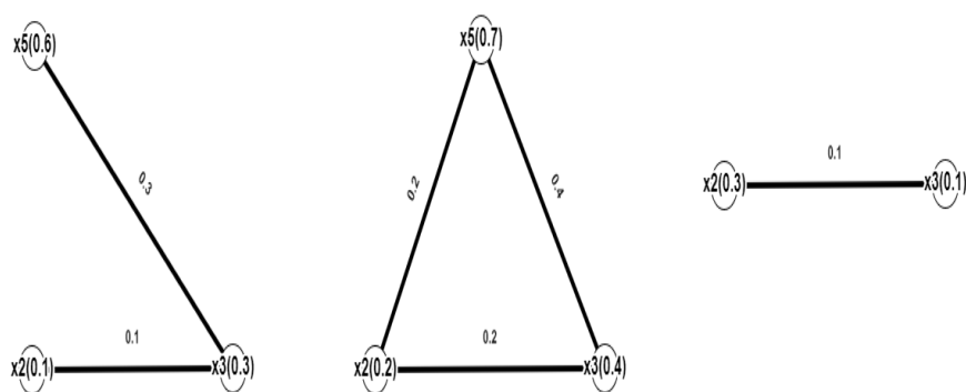
Figure 4. Representation of FH -Graph H
