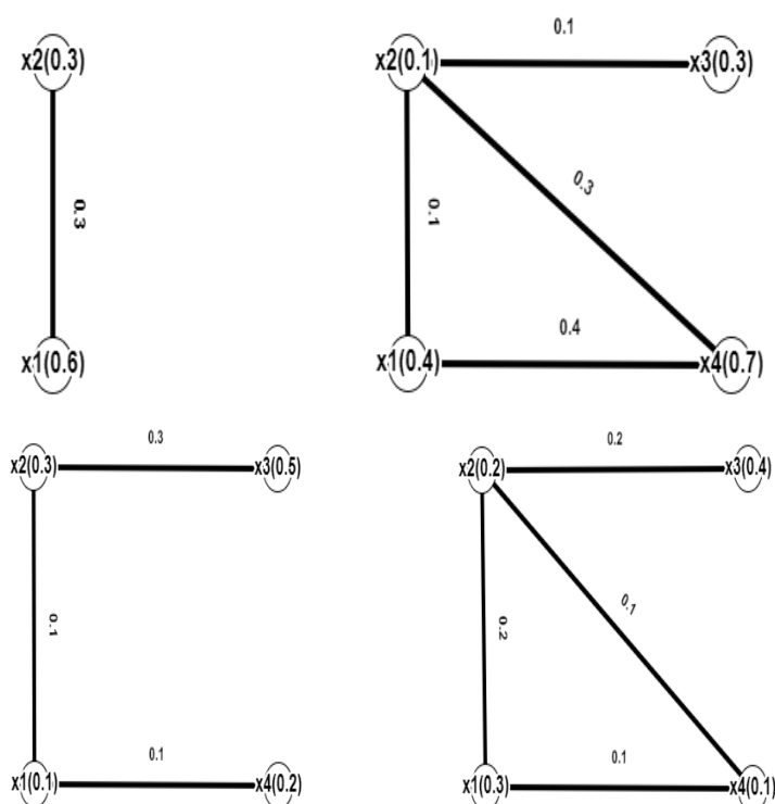
Figure 1. Representation of \mathbb{F} -hypersoft Graph
