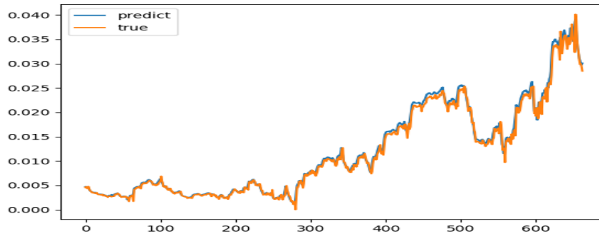
Figure 1. LSTM results.
