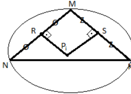
Figure 2: Centroids' circumcenter
