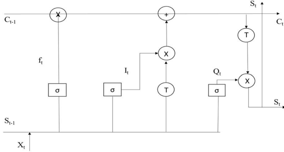
Figure 1. LSTM [13]
