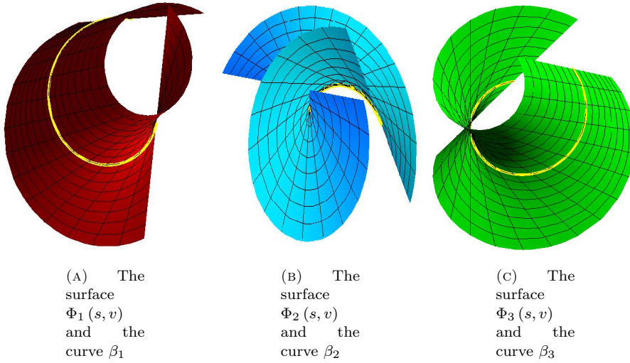
FIGURE 1. The spatial quaternionic Smarandache ruled surfaces (top view) and the quaternionic Smarandache curve (yellow) with s \in [-0.5, 1.5] and v \in [-1, 1]
