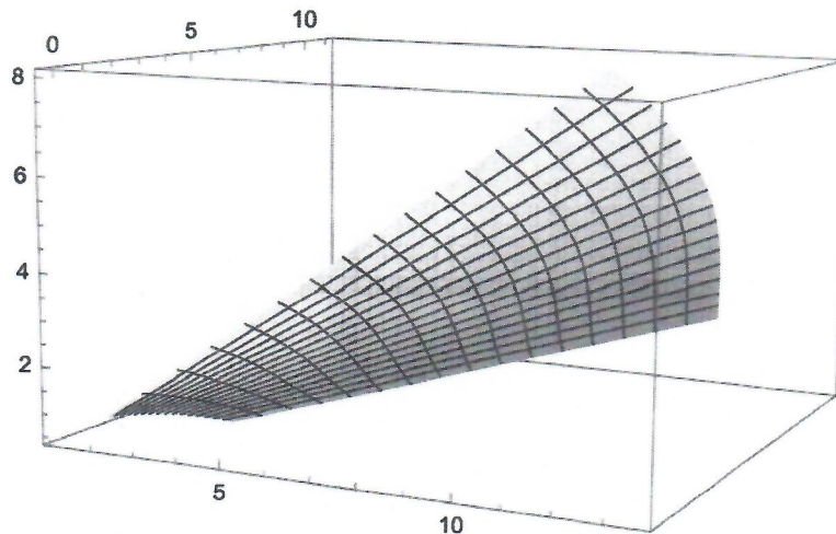
Figure 5: NB-equiform Smarandache ruled surface Y(\vartheta, v)
