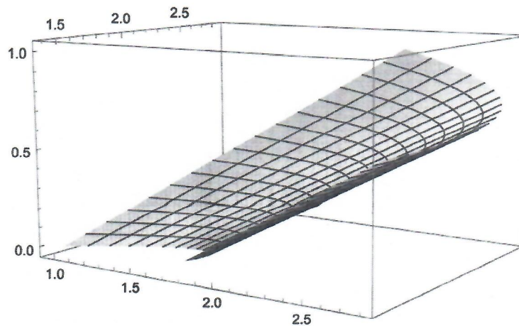
Figure 4: TB -equiiform Smarandache developable ruled surface \Theta(\vartheta, v)
