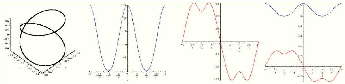
Fig. 2. The tangent indicatrix curve (black) and the curvature K_T (blue) and the torsion \tau_T (red)
