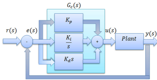
Fig. 2 PID controlled feedback system in the s domain
