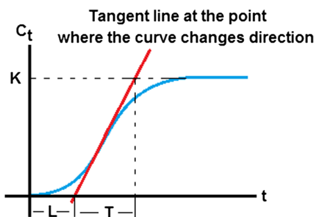
Fig. 3 Unit step response curve of a system
