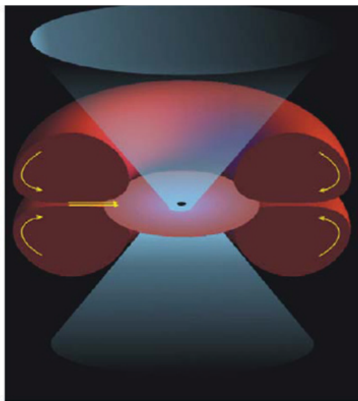
Fig. 1b. Dipole toroidal vortex in the AGN center: 3D picture. Cones sketch out the wind and radiation.
