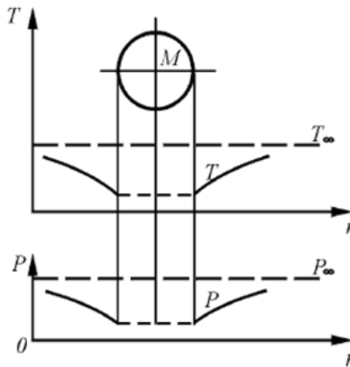
Fig. 5.17. Distribution of temperature and pressure around a conglomerate of toroidal vortices in free space
