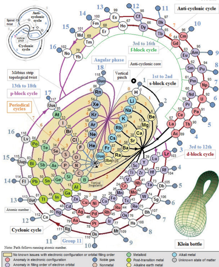
Figure 2. Klein-bottle inspired periodic table of elements (www.uvs-model.com)
