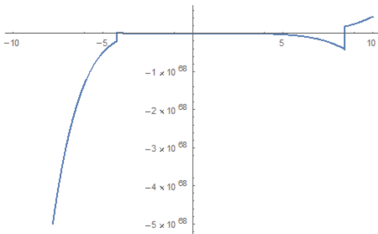
Figure 2. Plot of Ermakov-type solution for A=1 , B=-10
