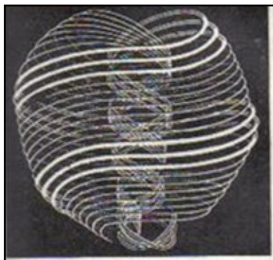
Fig.5 Kerr-Neumann Compton radius vortices
