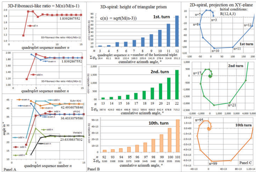
Figure 3. Evolution of 3D-spirals over n (which is time measured in generation units). Convergence is fast attained at n around 10. Panel A shows the 3D-tribonacci ratio M(n)/M(n-1) with limit \Phi_{3D} = 1.8393 attained from above (below) according to even (odd) n ; lower panel shows convergence of angles \varphi , \theta , and Euler-X. Panel B shows vertical evolution of spiral along Z-axis direction. Panel C shows projections of 3D-spiral upon XY-plane (similar but not identical to figure 1C). Shape of spiral in first turn depends on initial conditions R(12,4,3) . Some values of n are marked along spirals.
