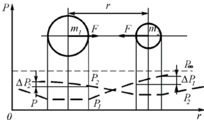
Fig. 10.1. Mechanism of gravitational interaction of two bodies: the change in temperature and pressure in proximity/vicinity/ neighborhood of a gravitational mass and gravitational interaction between the two masses
