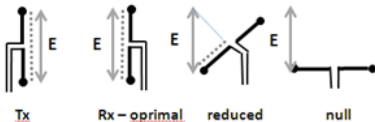
Figure 1, Comparison of conventional dipole transceiver antennas positioning.
