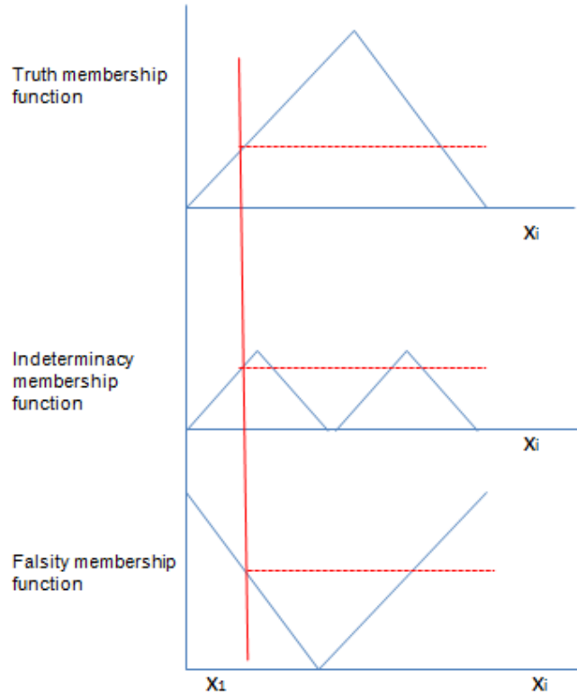
Fig. 2: Neutrosophication process [11]
