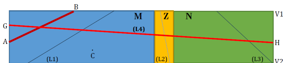
Figure 1: A Neutrosophic Model.
