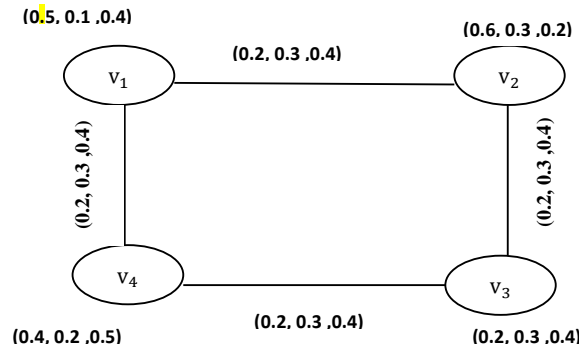
Figure 10: Constant SVN-graph.
