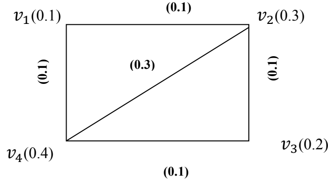
Figure 1: Fuzzy Graph
