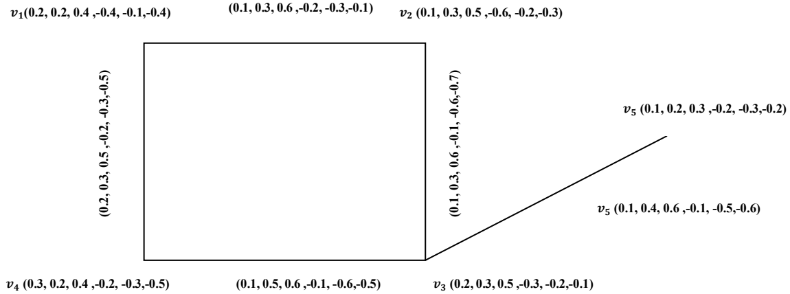
Fig. 7: Incident BSVN-graph
