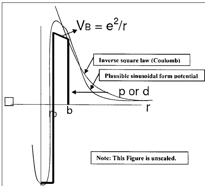
Figure 1. Potential for Coulomb barrier reversal for STTB, from Takahashi. 2
