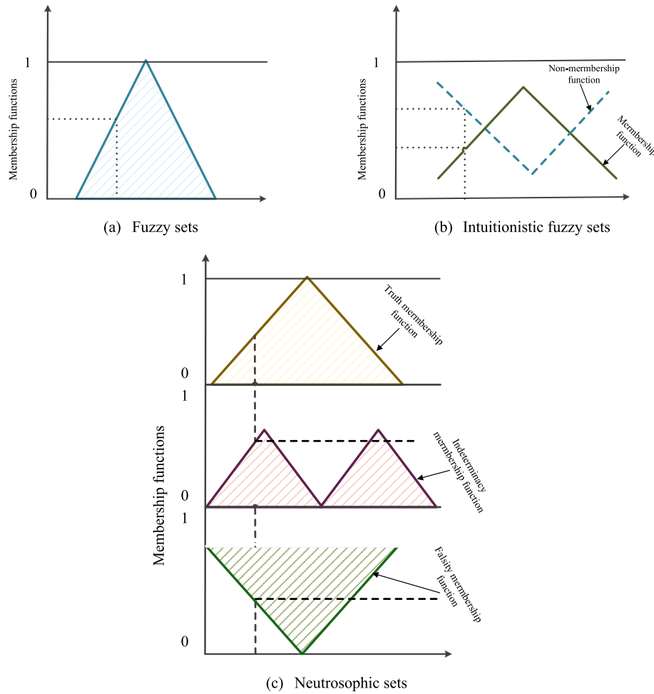
Fig. 2. Some fuzzy sets and their membership functions.
