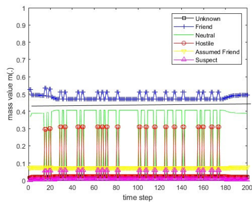
Figure 72. The values of the resulting belief mass for scenario 4 and the PCR5 rule for 3 BBAs.
