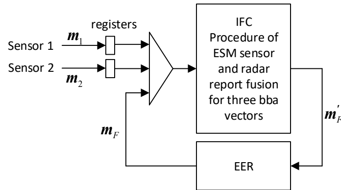
Figure 3. The diagram of the information-fusion process in the information-fusion center (IFC) for two sensors and electronic entity record from the IFC database. Explanations: \mathbf{m}_i , a BBA measure vector of i -th sensor; \mathbf{m}_F , a generalized BBA measure vector that is a part of the electronic entity record in the IFC; EER, an electronic entity record in the IFC database.
