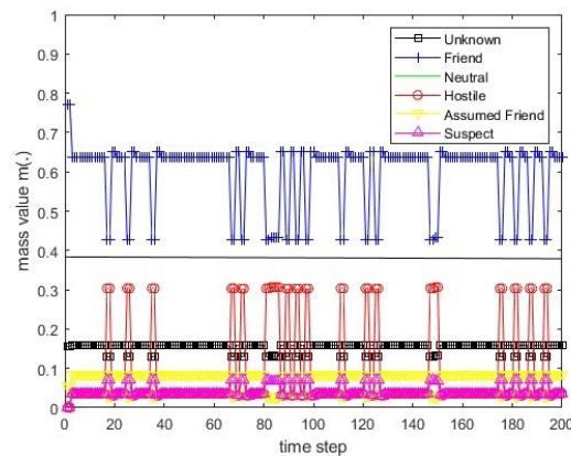
Figure 49. The values of the resulting belief mass for Monte Carlo scenario 5 and the PCR5 rule for 3 BBAs.
