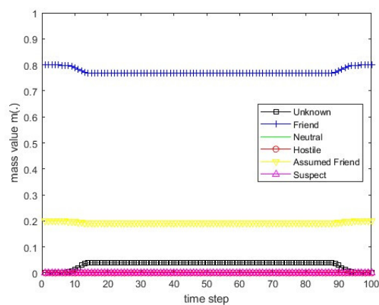
Figure 59. The course of scenario number 3 for sensor 2.
