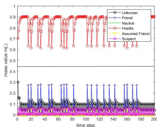
Figure 29. The values of the resulting belief mass for scenario 3 and the PCR5 rule for 2 BBAs.
