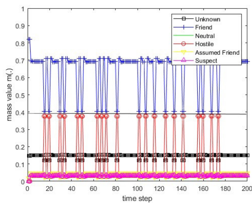
Figure 32. The values of the resulting belief mass for scenario 2 and the PCR5 rule for 3 BBAs.
