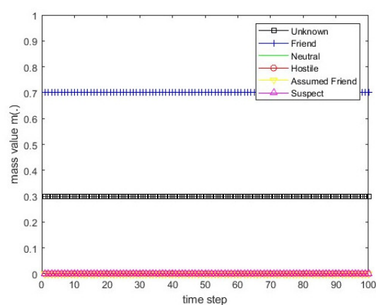
Figure 5. The course of scenarios number 1, 2, and 5 for sensor 1.
