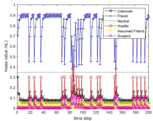
Figure 42. The values of the resulting belief mass for Monte Carlo scenario 6 and the PCR1 rule.
