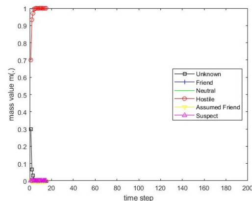
Figure 14. The values of the resulting belief mass for scenario 3 and Dempster's rule.
