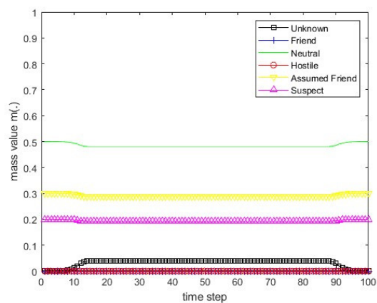
Figure 58. The course of scenario number 2 for sensor 2.
