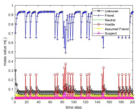
Figure 43. The values of the resulting belief mass for Monte Carlo scenario 5 and the PCR3 rule.
