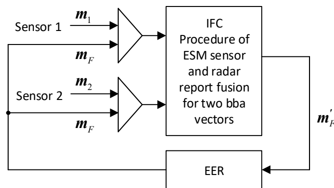
Figure 2. The diagram of the information-fusion process in the information-fusion center (IFC) for two sensors. Explanations: m_i a BBA measure vector of i -th sensor; m_F , a generalized BBA measure vector that is a part of the electronic entity record in the IFC; EER, an electronic entity record in the IFC database.
