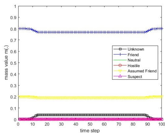
Figure 57. The course of scenario number 1 for sensor 2.
