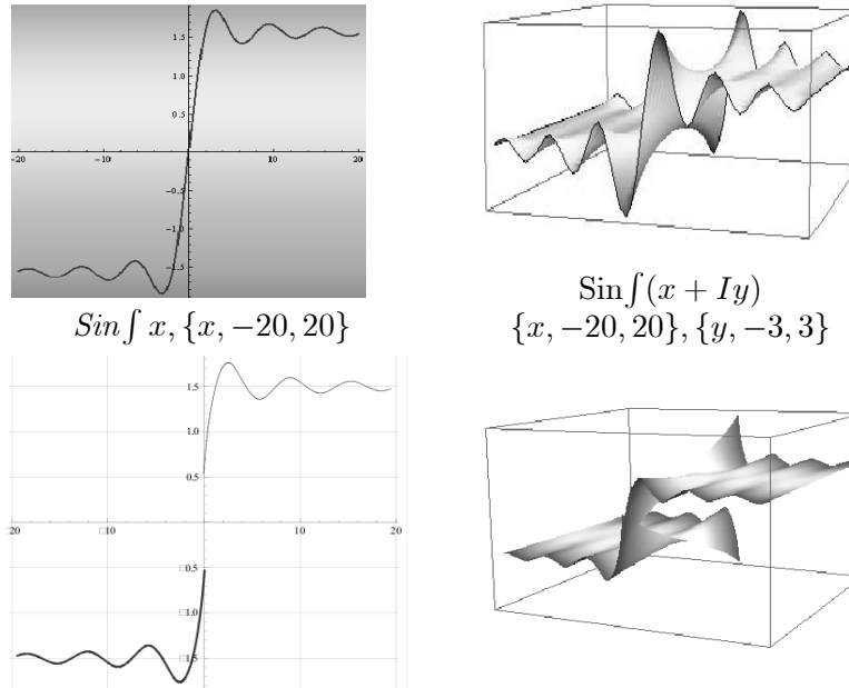
Figure 4: The graph of integral sine function \text{Si}(x) ▲ compared with the graph CE-SMF Eccentric amplitude 1.57aex[\theta, S(0.6; 0)] of eccentric variable \theta ▼
