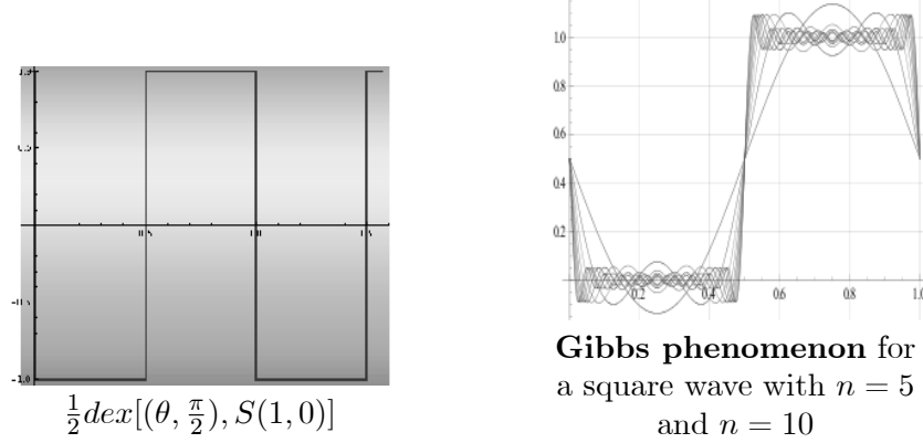
Figure 3: Comparison between the square function, eccentric derivative and its approximation by Fourier series expansion
