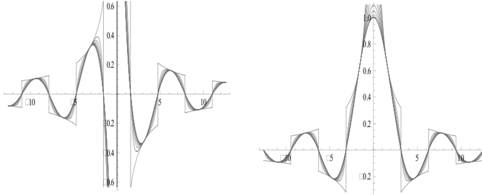
Figure 16: The graph of supermathematics cardinal cvadrilobe function ceqc(\theta) \blacktriangleleft and siqc(\theta) \blacktriangleright
