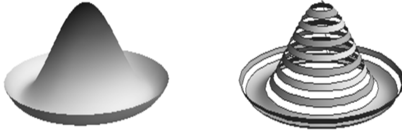
Figure 2: Cardinal sine function in 3D Mexican hat (sombrero)
