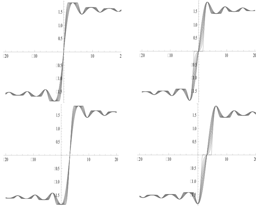
Figure 17: The graph of eccentric integral sine function sie_1(x)\blacktriangle and sie_2(x)\blacktriangledown
