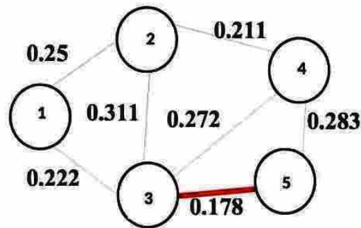
Figure (10): The selected edge (3,5) in G
